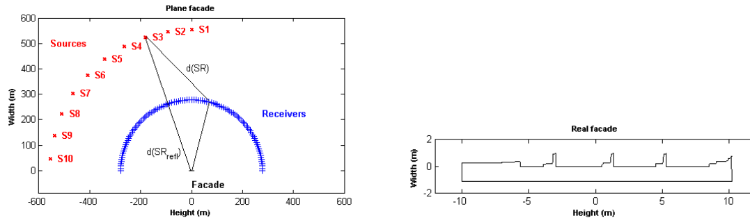
Fig. 2: Calculation set-up. Sources and receivers in far field conditions for a plane façade (left) and above a real building façade in Bordeaux (right).
