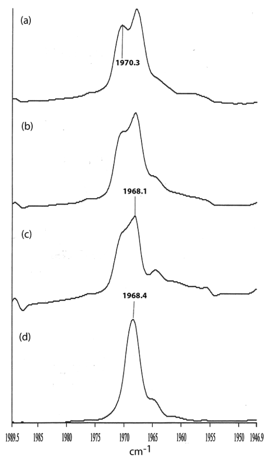
Figure 4. (a–c) 1968–1970 cm -1 band from the photolysis of 12bT/12bA in Ar matrix at 10 K (from Figure 2). (a) As obtained in Figure 2. (b) After 1 cycle of annealing to 30 K. (c) After 20 cycles of annealing to 30 K. (d) 1968 cm -1 band obtained after FVT of 12bT/12bA at 400 °C and isolation of the product in Ar matrix at 10 K.
