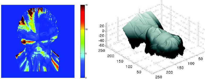
FIG. 3.4. Results on the 256 \times 256 'Beethoven' dataset. Left: squared error map of FM result; Right: reconstruction result of FM. The results of the FM scheme are qualitatively similar to the solution by Poisson reconstruction, though it as a much lower complexity. The left figure shows the difference from FM to the Poisson reconstruction, putting the latter into the role of the ground truth because of its overall higher accuracy.
