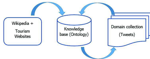
Figure 2. The arrows show how a resource is used. Wikipedia and tourism websites are used to populate the ontology; the ontology is used to help information extraction from the tweet collection and the additional extracted information is used to populate the ontology.
