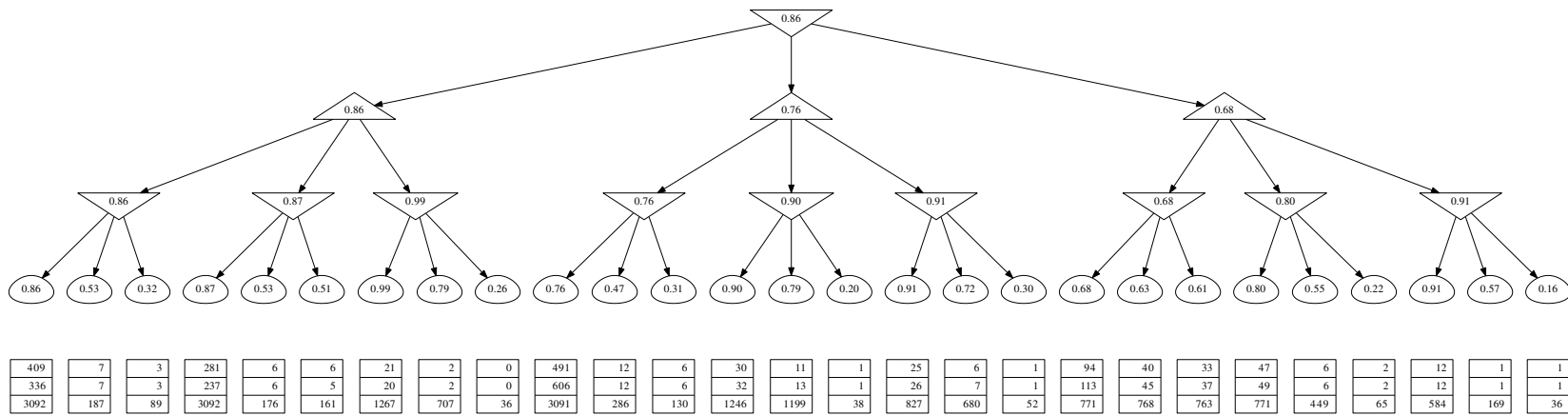
Figure 4: Our benchmark 3-way tree of depth 3. Shown below the leaves are the numbers of pulls of 3 algorithms: LUCB-MCTS (0.72% errors, 1551 samples), UGapE-MCTS (0.75%, 1584), and FindTopWinner (0%, 20730). Numbers are averages over 10K repetitions with \epsilon = 0 and \delta = 0.1 \cdot 27 .
