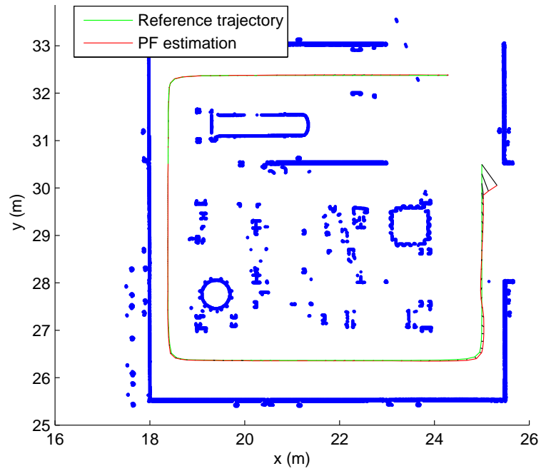
(a) Reference ( green ) and particle filter estimated ( red ) trajectory, cross section of environment ( blue )
