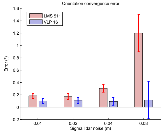
(b) Orientation convergence error
