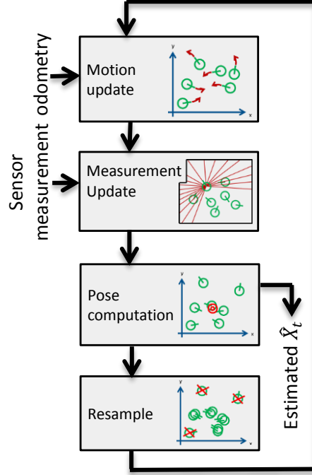
Figure 2: Main steps of particle filter-based localization
