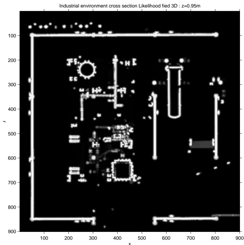
(d) Cross section of the resulting likelihood field (voxel unit). Lines in the figure correspond to horizontal bars of the fence that exist at z=0.95m
