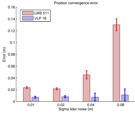
(a) Position convergence error
