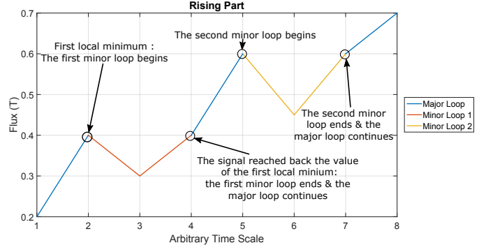
Figure 5: Arbitrary waveform (rising part) split into major and minor loops for core losses calculation
