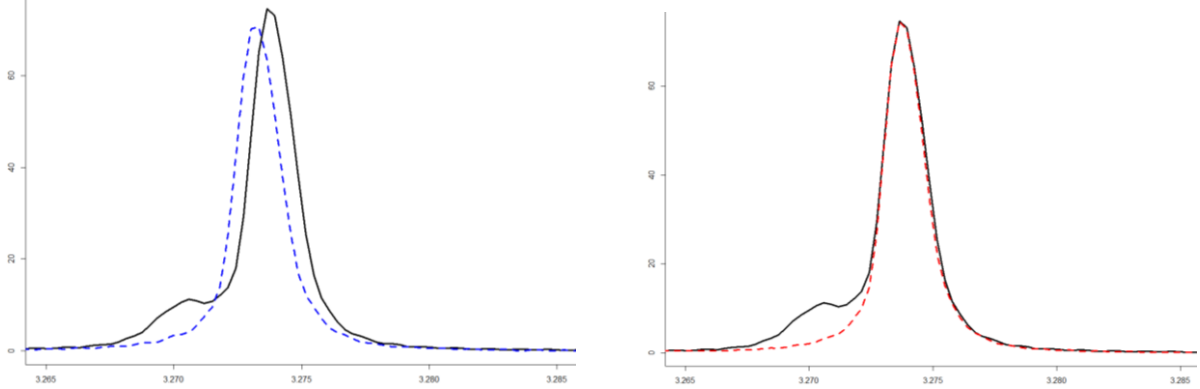
Figure 1. On the left in solid line, the main peak of the creatinine in the spectrum of the synthetic urine. In dotted line, the same peak observed on the spectrum of the creatinine before the warping stage. On the right in dotted line, the main peak of the creatine spectrum observed after the warping stage.
