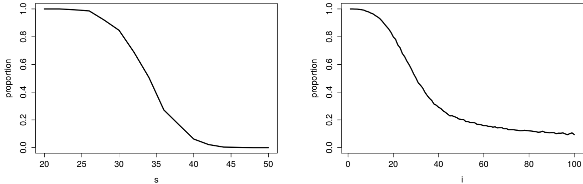
Figure 3: In this figure, \tilde{x} is a random vector such that \text{supp}(\tilde{x}) = \llbracket 1, s \rrbracket , with s \in \{20, 22, \dots, 50\} and |\tilde{x}_1| \geq \dots \geq |\tilde{x}_s| . For every s \in \{20, 22, \dots, 50\} , a sample of 500 families \mathcal{D} = \{d_1, \dots, d_{256}\} and 500 observations of the random vectors \tilde{x} have been simulated. For each family and observation of \tilde{x} , we compute the solution x^{\text{bp}} of the basis pursuit problem \mathcal{P}_1 . On the left panel, we have the representation of the proportion of times when x^{\text{bp}} = \tilde{x} as a function of s . One notices that when s \geq 45 , the event x^{\text{bp}} = \tilde{x} is never observed. In the right panel, we set s = 50 and r is a permutation of \llbracket 1, 100 \rrbracket such that |x_{r(1)}^{\text{bp}}| \geq \dots \geq |x_{r(100)}^{\text{bp}}| (by lemma 3, \text{Card}(\text{supp}(x^{\text{bp}})) \leq 100 ). For each i \in \llbracket 1, 100 \rrbracket in the x -axis, the y -axis represents the proportion of times for which r(i) \in \text{supp}(\tilde{x}) . Note that largest components of x^{\text{bp}} are elements of \text{supp}(\tilde{x}) .
