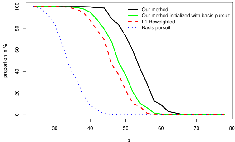
Figure 6: The performances of the basis pursuit, l^1 reweighted and our method are represented by the proportions of realisations of the events x^{\text{bp}} = \tilde{x} , x^{11,(8)} = \tilde{x} and x^{(8)} = \tilde{x} as a function of the number of non null components of \tilde{x} denoted s . In these simulations, our method is initialized with two different point: x^{(0)} given by the algorithm described in figure 4 and x^{\text{bp}} the basis pursuit solution.
