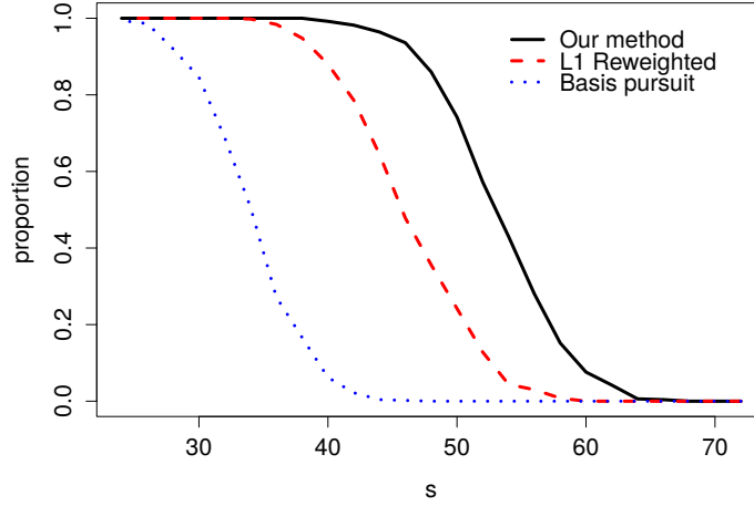
Figure 4: The performances of the three competing methods are represented by the proportions of realisation of the events x^{\text{bp}} = \tilde{x} , x^{11,(8)} = \tilde{x} and x^{(8)} = \tilde{x} as a function of the number of non null components of \tilde{x} denoted s . One notices that the graph of the reweighted l1 minimization method is almost the same as those given in [9].
