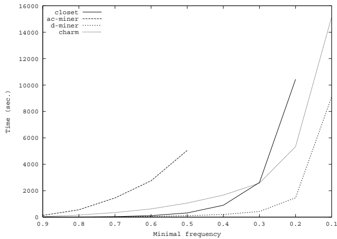
Figure 6: Connect4
