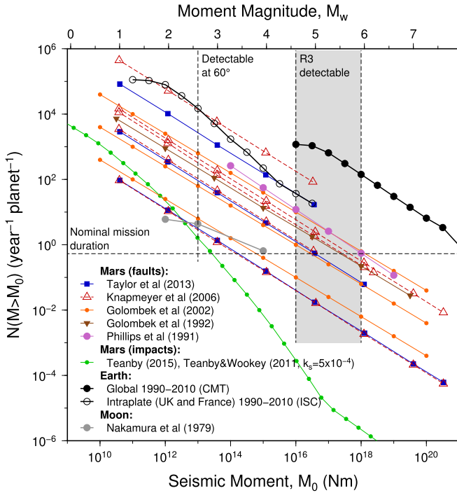
Fig. 3 Predictions of martian seismicity for faults and impacts. Mars faulting estimates are based on Phillips (1991), Golombek et al. (1992), Golombek (2002), Knapmeyer et al. (2006) (global) and Taylor et al. (2013) (Cerberus Fossae only). Impact seismicity is based on Teanby (2015)’s nominal regional estimates and Teanby and Wookey (2011)’s global estimates with a revised seismic efficiency of k = 5 \times 10^{-4} . For comparison the seismicity is also shown for the Moon (Nakamura et al. 1979) and Earth (whole globe from Harvard CMT catalogue and Intraplate settings from ISC catalogue). The dashed vertical line shows the threshold magnitude for a detection at 60^\circ offset based on the InSight seismometer performance and waveform modeling (Teanby and Wookey 2011). The grey shaded area shows the threshold magnitude for detection of the R3 surface wave, which will allow source-receiver distance calculations (Panning et al. 2015). Horizontal dashed line indicates mission duration of 1 Mars year (2 Earth years)
