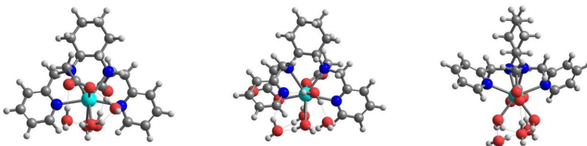
Figure 2. DFT optimized geometry of the Y^{3+} analogue of the Eu^{3+} .
