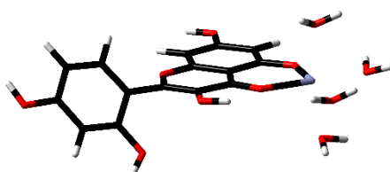
Figure 2. Solvation sphere around zinc cation bound to morin.
