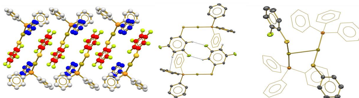
Figure 1. Examples showing \pi stacking (Compound 1 ), C-H...F bond (Compound 6 ) and aurophilic interaction (Compound 8 ).
