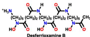
Figure 1. Chemical formula of desferrioxamine B.
