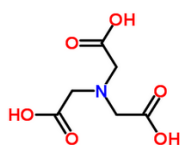
Figure 1. Nitrilotriacetic acid (NTA).
