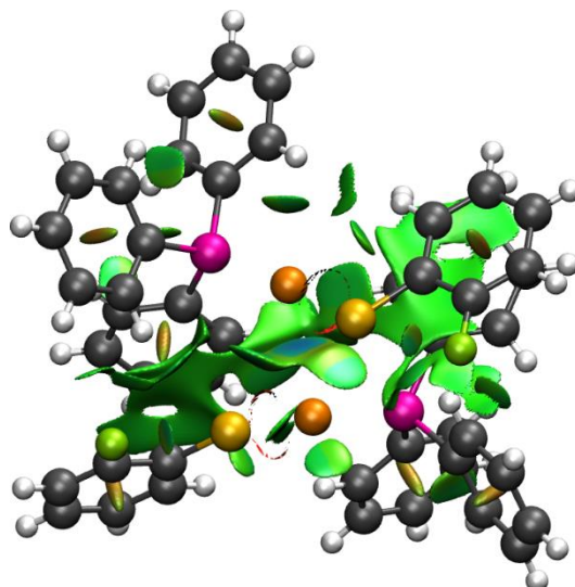
Figure 2. General view of the NCIPLOT interaction analysis in compound 8 . Auophilic attractive interaction could be noted as blue colored surface. Code: Au: golden, F: green, S: yellow, P: orange, C: gray and H: white.
