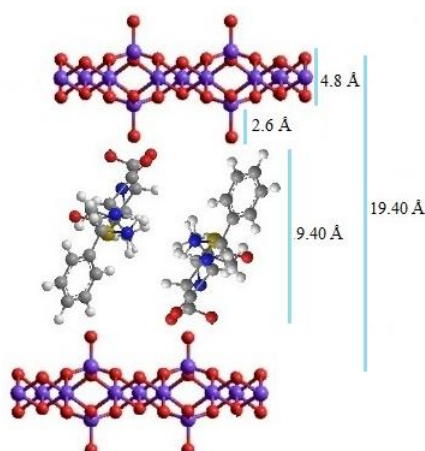
Figure 1. Spatial orientation of amoxicillin after intercalation.
