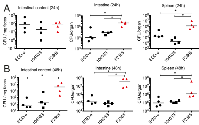
Fig. 1. Comparative virulence of lineage I strain F2365 and lineage II Listeria monocytogenes strains EGD-e and 10403S. cfu counts in the intestinal content, intestine, and spleen of BALB/c mice were measured at 24 h (A) and 48 h (B) after intragastric inoculation with 5 \times 10^9 bacteria of the indicated strains. Each dot represents the value for one mouse. Statistically significant differences were evaluated by the Mann–Whitney test. * P < 0.05 .
