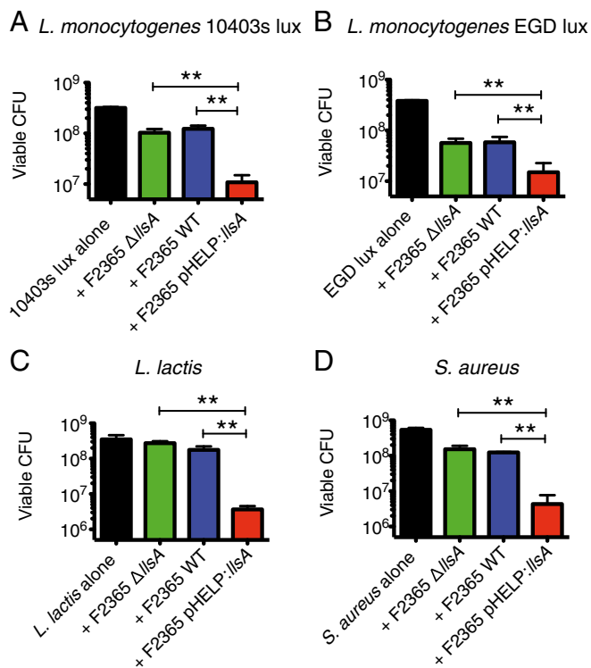
Fig. 4. LLS inhibits the growth of other bacteria in vitro. Viable L. monocytogenes 104035 lux (A), L. monocytogenes EGD lux (B), L. lactis (C), and S. aureus (D) at 24 h postinoculation either alone or in coculture with L. monocytogenes F2365 pHELP:LLS compared with L. monocytogenes F2365 WT or L. monocytogenes F2365 \Delta llsA . Data from three independent experiments are presented. Error bar shows SD. Data were analyzed by using a Student's t test. *** P < 0.01.
