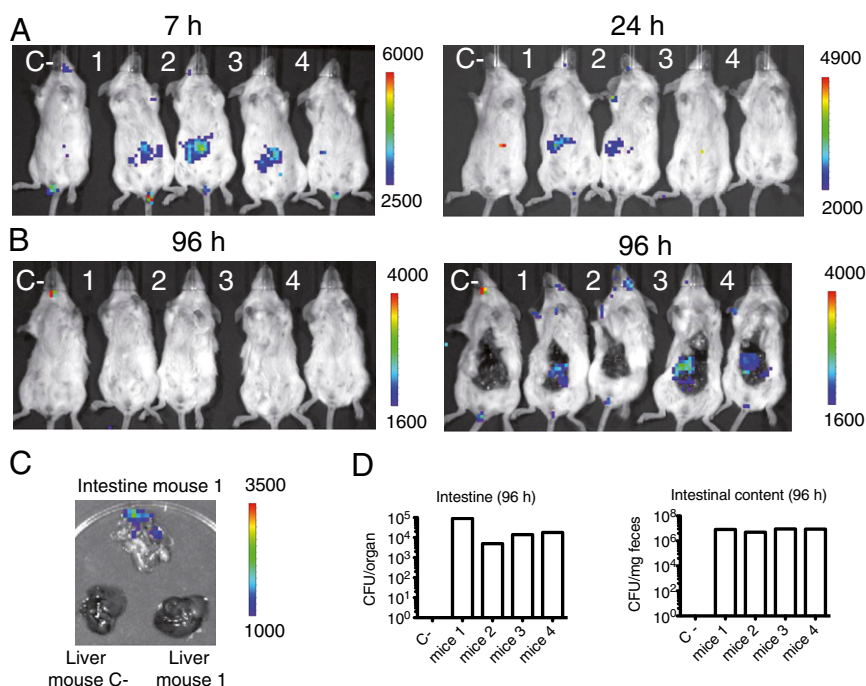
Fig. 3. Bioluminescence imaging of LLS promoter induction. (A) Induction of LLS promoter in the abdominal region after intragastric inoculation of four mice with 5 \times 10^9 bacteria per BALB/c mouse. C, control mouse noninfected. Images were acquired at the indicated hours after infection with an IVIS Spectrum Imaging System. (B) Induction of LLS promoter specifically in the intestine of the same mice as in A but at 96 h p.i. Images were taken before (Left) and after (Right) abdominal skin and peritoneum dissection. (C) Ex vivo imaging of the liver and intestine removed from the mice in B. (D) Bacterial counts in the intestinal tissue (intestine) and intestinal luminal content of the same mice at 96 h p.i.
