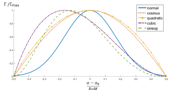
Figure 2 – normalized force-length relationship suggested by the 5 mathematical models
