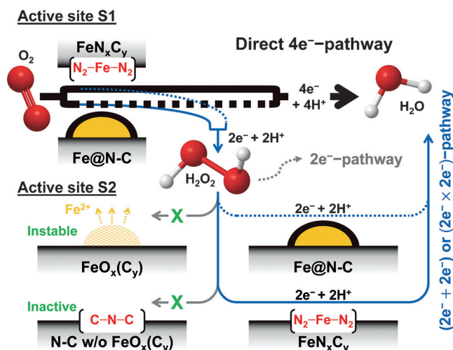
Figure 4. ORR mechanisms on Fe-N-C catalysts in acid medium. The site S1 is FeN x C y moieties or Fe@N-C. FeN x C y mostly catalyzes direct 4e - ORR, but also releases a minor fraction of H 2 O 2 . Fe@N-C produces higher fraction of H 2 O 2 in comparison to FeN x C y . The released H 2 O 2 is then reduced to H 2 O on site S2 (either FeN x C y or Fe@N-C). Surface-exposed Fe particles and N-groups without subsurface Fe are PRR-inactive.
