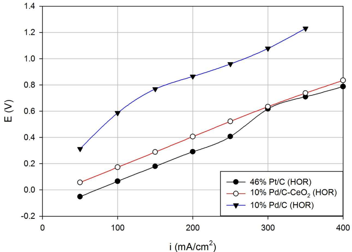
Figure 6. Polarization curves of hydrogen pumping tests comparing the HOR performance of Pd/C-CeO 2 to both Pd/C as well as Pt/C.
