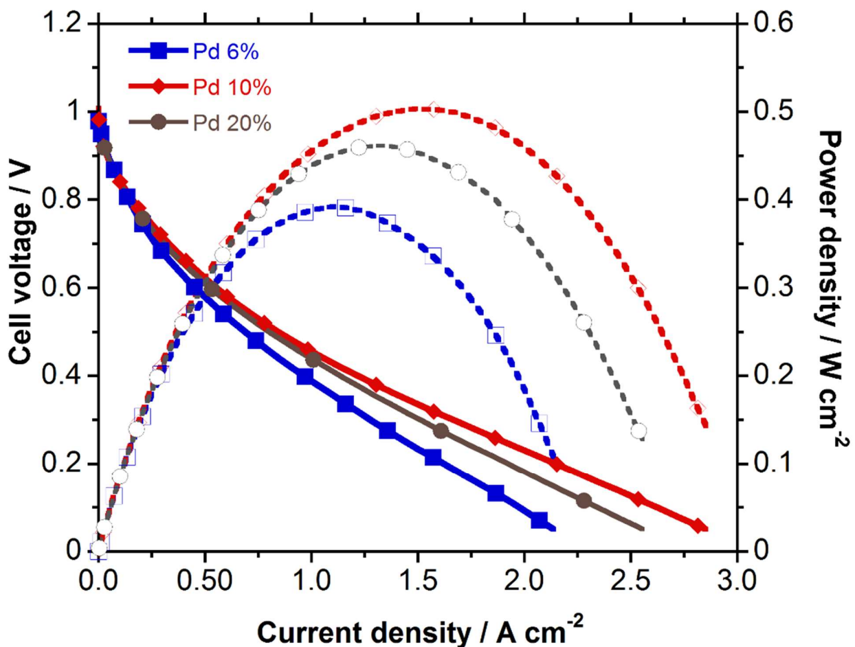
Figure 5. Polarization curves of AEM-FCs using Pd/C-CeO 2 anode catalysts with 10wt% Pd,[16] 6%Pd and 20wt%.
