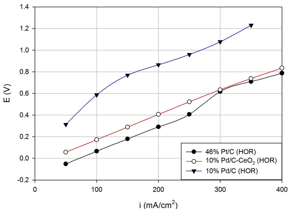
Figure 6. Polarization curves of hydrogen pumping tests comparing the HOR performance of Pd/C-CeO 2 to both Pd/C as well as Pt/C.
