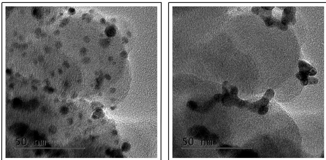
Figure 12. Selected ILTEM micrographs of the Pd/C sample in (A) its pristine state, and (B) after 1000 CV cycles in 0.1M NaOH at 25°C.
