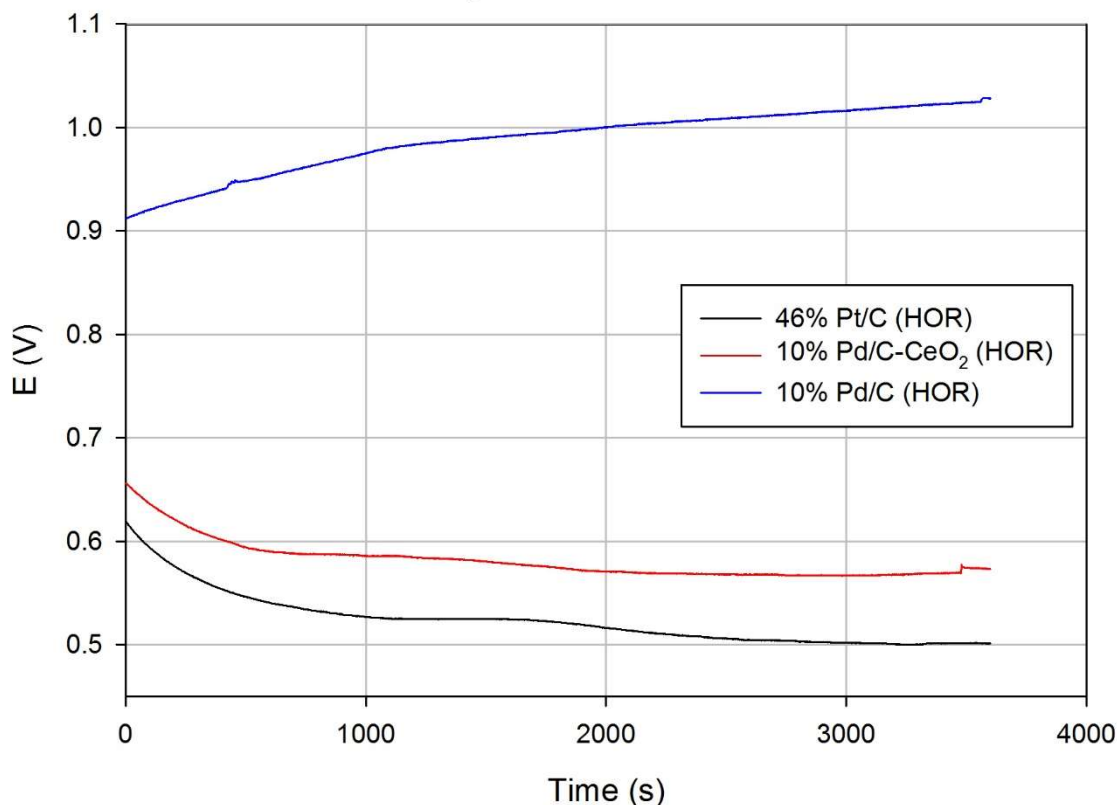
Figure 7. Stability run of hydrogen pumping tests of Pd/C-CeO 2 catalyst as compared to both Pd/C and Pt/C under 300mA cm -2 steady state operation.
