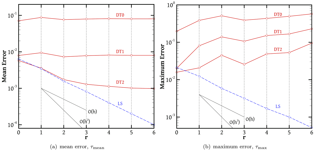
Figure 16: The mean (a) and maximum (b) errors (Eqs. (19) and (20)) of the DT (red solid lines) and LS (blue dashed lines) gradient schemes applied on the function \phi = \tanh(x) \tanh(y) on the series of globally distorted grids (Fig. 15). For the DT method, the number of corrector steps n is indicated on each curve as DT n .
