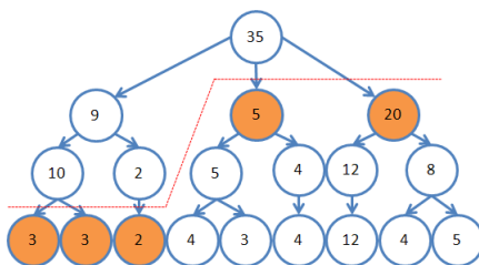
Figure 1: Dynamic programming works as follows: the energy at any node S is compared to the sum of the energies of the children. If \omega(S) \leq \sum \omega(T_k) , T_k children of S , one keeps the class S ; if not, one replaces S by its sons. The optimal cut is then the union of the remaining classes. It results here in the partition in dotted lines.
