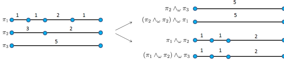
Figure 6: Hierarchy with three levels. The energies of the classes are indicated. Those of the partial partitions are obtained by sums of their classes. the \wedge_\omega of the three partitions is not (\pi_2 \wedge_\omega \pi_3) \wedge_\omega \pi_1
