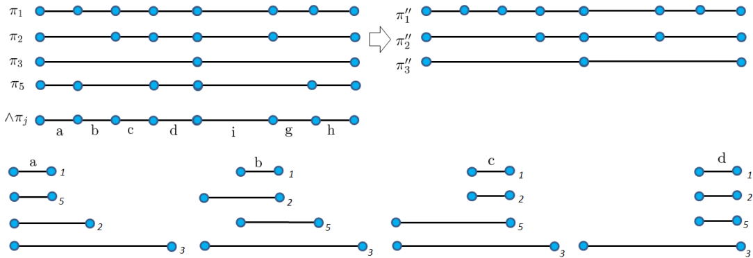
Figure 8: Four cuts \pi_j in an unknown braid of an unknown partial monitor H'' . The associated cones allow to find the three levels \pi_j'' of H'' .
