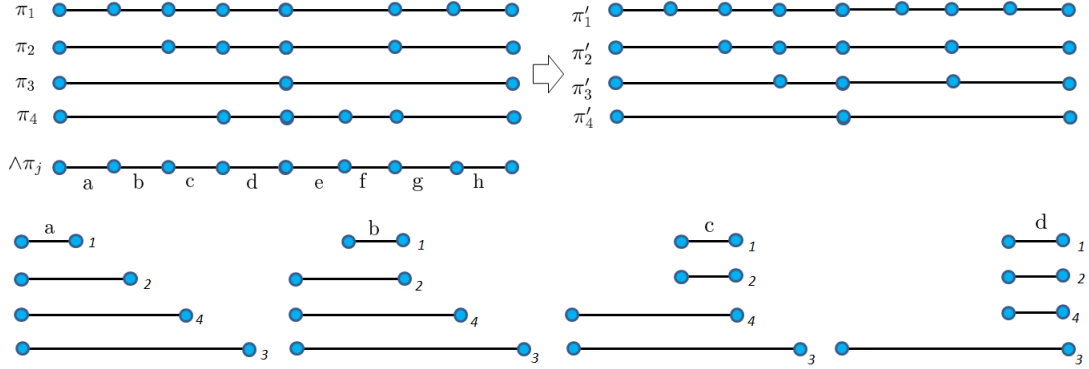
Figure 7: Four cuts \pi_j in an unknown hierarchy H' . The associated cones allow to find the four levels \pi'_j of H' .
