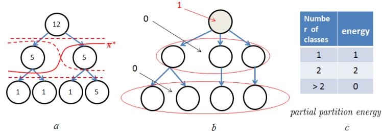
Figure 5: a) in case of \vee -composition, there is a unique minimal cut \pi^* and its energy is minimal, but other cuts have also the same energy. b) and c) depict a non h -increasing energy \omega(\pi) which depends on the number of classes of the p.p. \pi . The two cuts surrounded by ellipses are minimal (hence no energetic lattice), and none of them is obtained by dynamic program, which gives the cut in grey.
