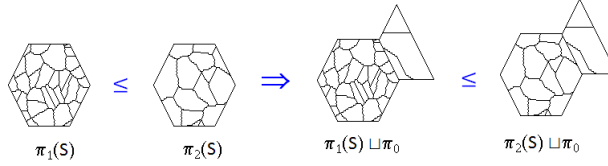
Figure 3: Hierarchical increasingness
