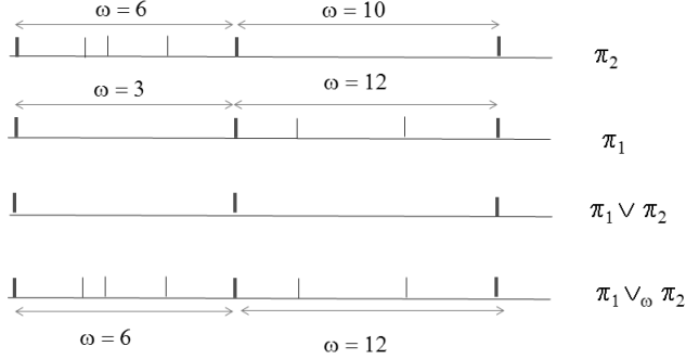
Figure 4: The energetic ordering induces a lattice where one takes the less energetic partial partition in each class of \pi_1 \vee \pi_2 (here for a hierarchy).
