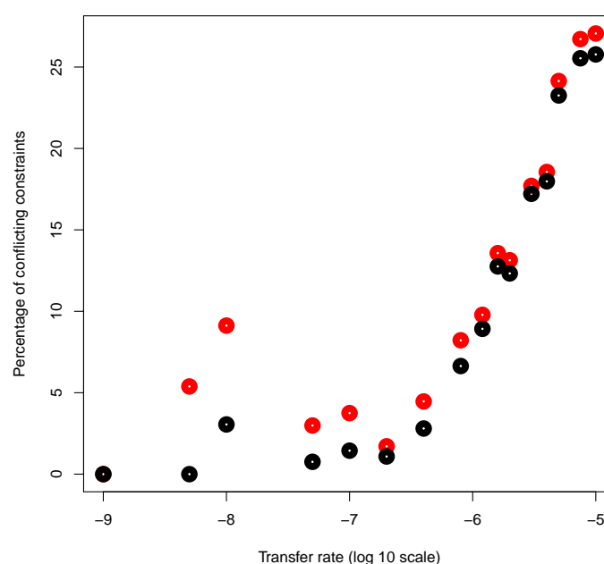
Figure 3: Fraction of constraints that have to be removed in order to get a time compatible set, as a function of the transfer rate ( \log_{10} scale). Red dots are for the fraction of constraints in conflict with the true (simulated) tree, and black dots are for the fraction of constraints in conflict with the reconstructed tree, minimizing the conflicts.
