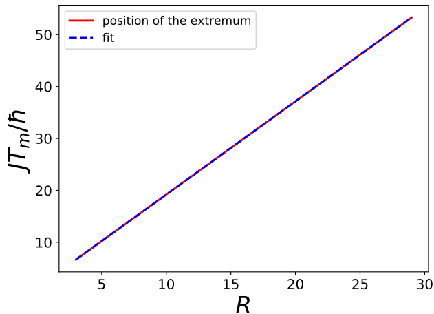
Figure S4. Trajectory of an extremum of the connected spin-spin correlation function for the LRTI model (lin-lin scale). It corresponds to the dashed, dark blue line in Fig. 2(b) of the main paper. The figure shows the numerical results found from Fig. S3 (solid red line) together with a fitted power law (dashed blue line).
