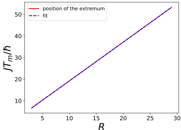
Figure S4. Trajectory of an extremum of the connected spin-spin correlation function for the LRTI model (lin-lin scale). It corresponds to the dashed, dark blue line in Fig. 2(b) of the main paper. The figure shows the numerical results found from Fig. S3 (solid red line) together with a fitted power law (dashed blue line).
