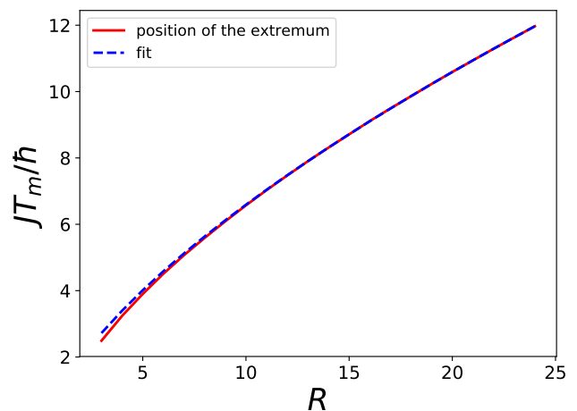
Figure S2. Trajectory of the first extremum of the connected spin-spin correlation function for the LRXY model (lin-lin scale). The figure shows the numerical results found from Fig. S1 (solid red line) together with a fitted power law (dashed blue line).
