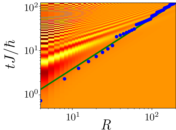
Figure S1. Spreading of the connected spin-spin correlation function for the LRXY model with \alpha = 2.3 (same data as in Fig. 2(a) of the main paper; log-log scale). The filled blue points correspond for each distance R to the first time where the correlation reaches 2% of its maximum value. The solid green line shows the power law predicted theoretically with a fitted multiplicative factor.
