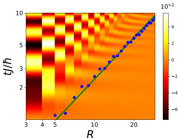
Figure S3. Spreading of the connected spin-spin correlation function for the LRTI model with \alpha = 1.7 (same data as in Fig. 2(b) of the main paper; log-log scale). The filled blue points correspond for each distance R to the first time where the correlation reaches 2.8% of its maximum value. The solid green line shows the power law predicted theoretically with a fitted multiplicative factor.
