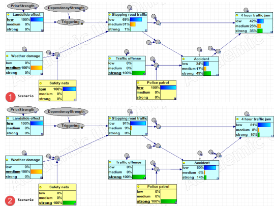
Fig. 6. Ground Bayesian network obtained by unrolling the PRM of Figure 4 on the instance given in Figure 5, with two scenarios of probabilistic inference.
