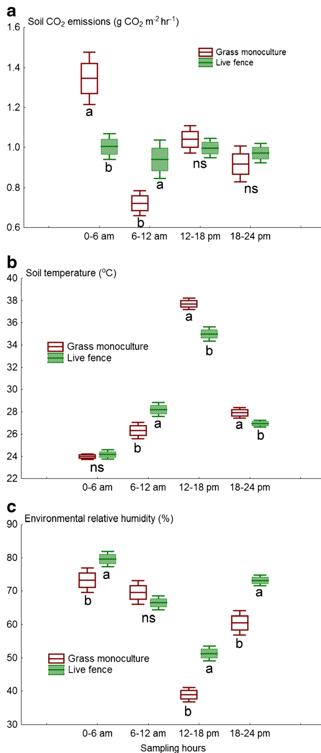
Fig. 4 a Fluctuations of soil CO 2 emissions at four different times of the day. b Soil temperature (0- to 5-cm depth). c Environmental relative humidity at 1-m height, measured in livestock systems with live fences (LF) and livestock systems in grass monoculture (GM). Soil CO 2 emissions are expressed in g m -2 h -1 , soil temperature in °C, and environmental relative humidity in %. Box plots represent means, while vertical bars represent standard error per time and system. ANOVA (Tukey test p \leq 0.05 ) was performed; different letters in each box at the same time of the day denote significant differences between means. ns no significant differences. Each column represents the mean of nine replications
