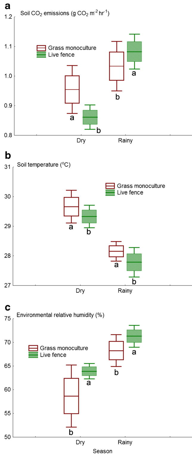
Fig. 3 a Seasonal variation of soil CO 2 emissions. b Soil temperature (0- to 5-cm depth). c Environmental relative humidity at 1-m height, measured in livestock systems with live fences (LF) and livestock systems in grass monoculture (GM). Soil CO 2 emissions are expressed in g m -2 h -1 , soil temperature in °C, and environmental relative humidity in %. Box plots represent means, while vertical bars represent standard error per season and system. ANOVA (Tukey test p \leq 0.05 ) was performed; different letters in each box of the same season indicate significant differences between means. ns no significant differences. Each column represents the mean of nine replications
