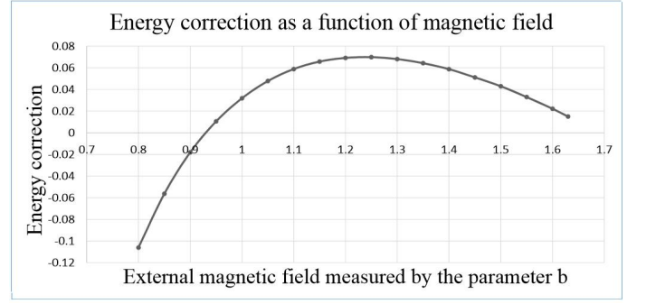
FIG. 1. Energy correction C_2(b) from (II.3) as a function of magnetic field, measured by the parameter b , cf (I.2).
