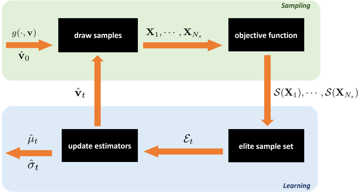
Figure 3 Schematic representation of the CE algorithm for optimization.
