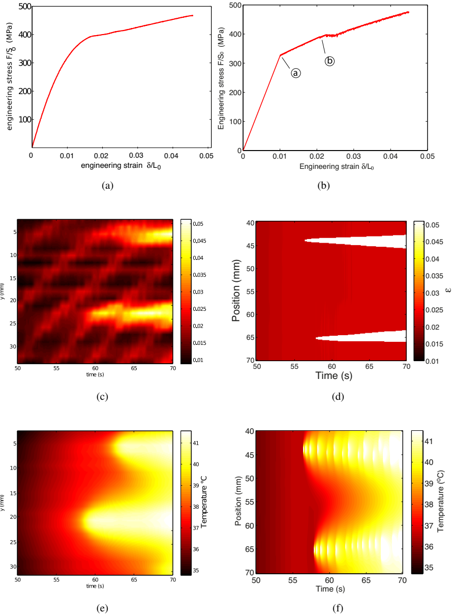
Figure 9: Comparison experiments / modelling: a/b- tensile curves at \dot{\delta}/L_0 = 4.2 \times 10^{-4} \text{ s}^{-1} . c/d- spatiotemporal map of axial deformation. e/f- spatiotemporal map of temperature. Dimensions are given in mm.
