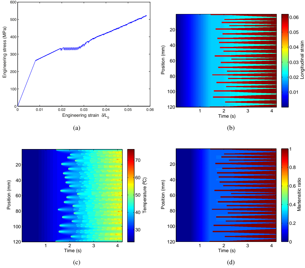
Figure 15: Modelling results at \dot{\delta}/L_0=1.4 \times 10^{-2} \text{ s}^{-1} : a-Engineering stress-strain curve; b/c/d spatiotemporal evolution of the longitudinal strain \varepsilon , temperature T (Celsius degrees), and of the martensite volume ratio f .
