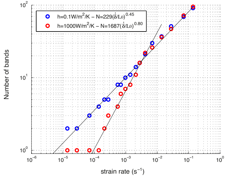
Figure 20: Number of localised band ( N ) vs. strain rate ( \dot{\delta}/L_0 ) in a log-log grid for two extreme convection conditions.
