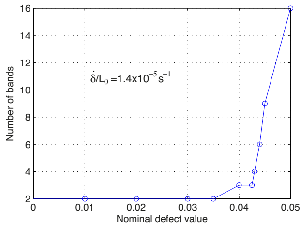
Figure 21: Effect of parameter \zeta as defect parameter on number of bands.
