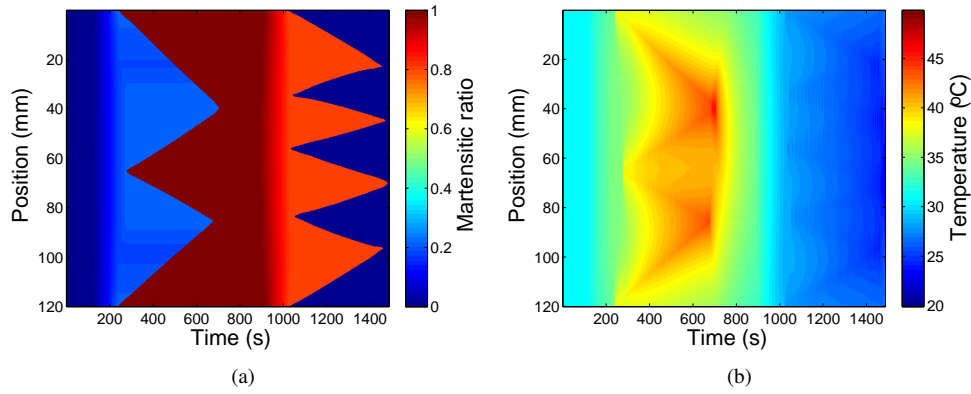
Figure 30: Modelling of martensite ratio (a) and temperature during the load-unload test at \dot{\delta}/L_0 = 8.3 \times 10^{-5} \text{ s}^{-1}
