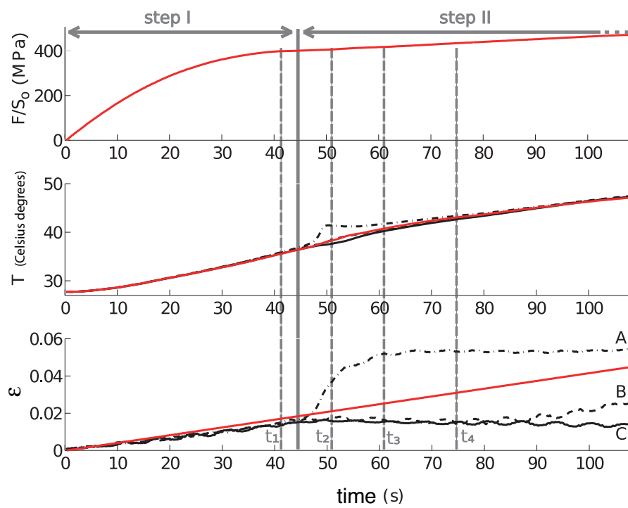
Figure 4: Simultaneous evolution of stress, temperature and longitudinal strain. Red lines are macroscopic quantities whereas dotted lines are local quantities at the three physical points (A,B,C) - at \dot{\delta}/L_0 = 4.2 \times 10^{-4} \text{ s}^{-1} .
