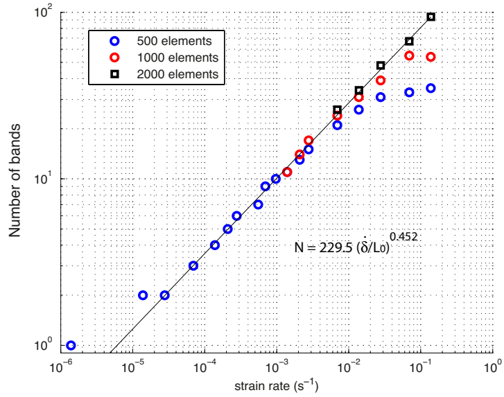
Figure 17: Number of localized band ( N ) vs. strain rate ( \dot{\delta}/L_0 ) in a log-log grid.
