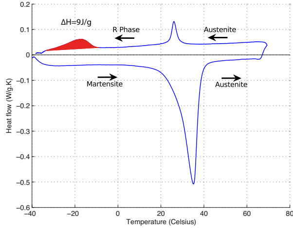
Figure 1: Differential Scanning Calorimetry of a Ni_{49.75} \text{ at\%Ti} .
