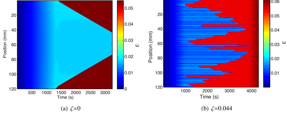
Figure 22: Illustration of bands for two different values of parameter \zeta .
