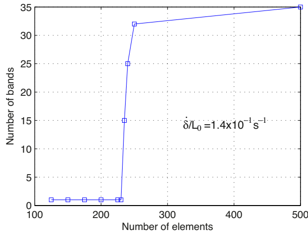
Figure 18: Effect of number of elements on number of bands.
