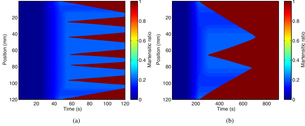
Figure 11: Modelling: spatiotemporal map of martensite ratio corresponding to IRIC test at: (a) \delta/L_0 = 4.2 \times 10^{-4} \text{ s}^{-1} ; (b) \delta/L_0 = 8.3 \times 10^{-5} \text{ s}^{-1} .
