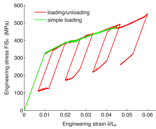
Figure 32: Modeled stress-strain curve obtained for incremental loading at \dot{\epsilon} = 4.2 \times 10^{-4} \text{ s}^{-1}
