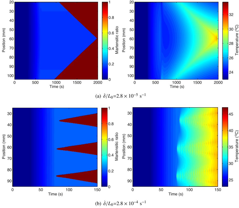
Figure 14: Modelling results: spatiotemporal evolution of the martensite volume ratio f and of the temperature T (Celsius degrees) at different strain rates for the exact same thermal conditions.
