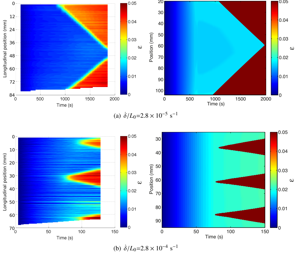
Figure 13: Comparison experiments / modelling of spatiotemporal evolution of the axial deformation at different strain rates for the exact same thermal conditions and geometries.
