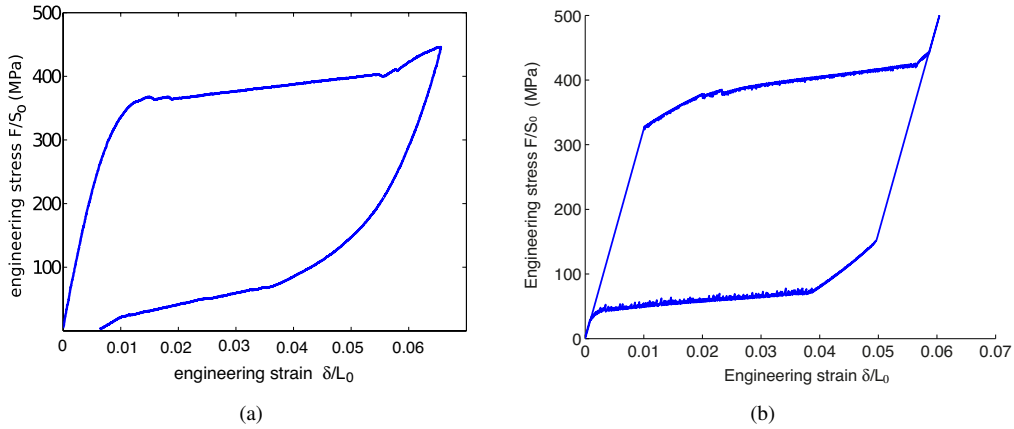
Figure 29: Experimental (a) vs. modelling (b) of load-unload curve at \dot{\delta}/L_0 = 8.3 \times 10^{-5} \text{ s}^{-1} .
