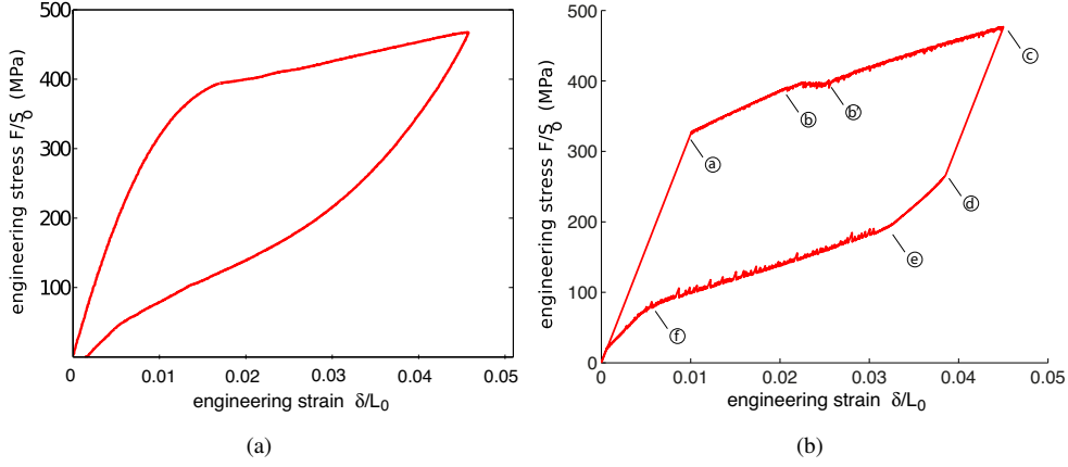
Figure 27: Experimental (a) vs. modelling (b) of load-unload curve at \dot{\delta}/L_0 = 4.2 \times 10^{-4} \text{ s}^{-1} .
