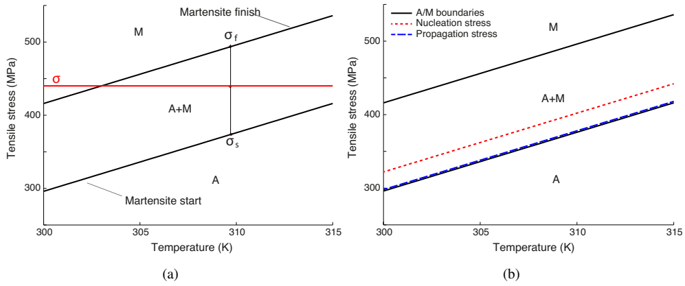
Figure 7: (a) Clausius-Clapeyron diagram and associated lever rule. (b) Homogeneous and localisation boundaries for the direct transformation: from A to M phases.
