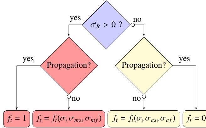
Figure 26: Calculation of the driving force depending on M transformation (direct), and or A transformation (reverse).
