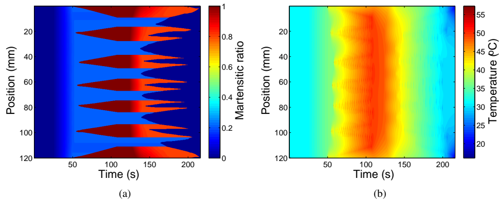
Figure 28: Modelling of martensite ratio (a) and temperature during the load-unload test at \dot{\delta}/L_0 = 4.2 \times 10^{-4} \text{ s}^{-1}
