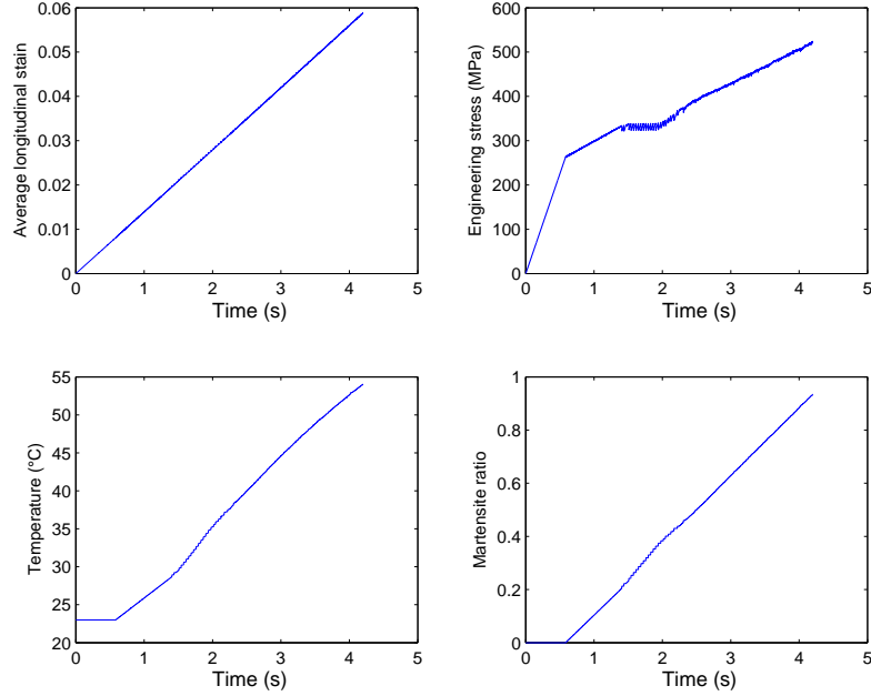
Figure 16: Modelling results at \dot{\delta}/L_0=1.4 \times 10^{-2} \text{ s}^{-1} : variation of engineering stress and strain, average temperature and martensite ratio as function of time.
