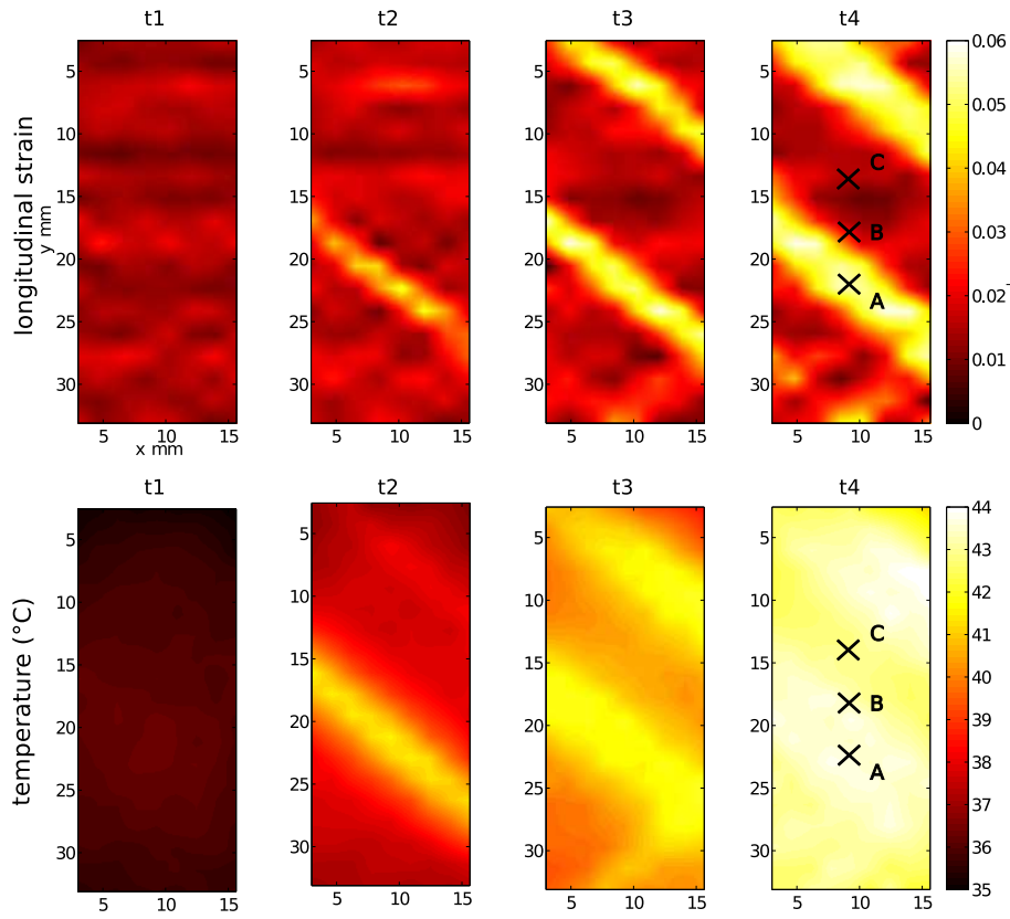
Figure 5: Temperature and longitudinal strain fields at four typical instants ( t_1 = 42 sec, t_2 = 51.25 sec, t_3 = 61.25 sec, t_4 = 75 sec) - at \delta/L_0 = 4.2 \times 10^{-4} \text{ s}^{-1} .
