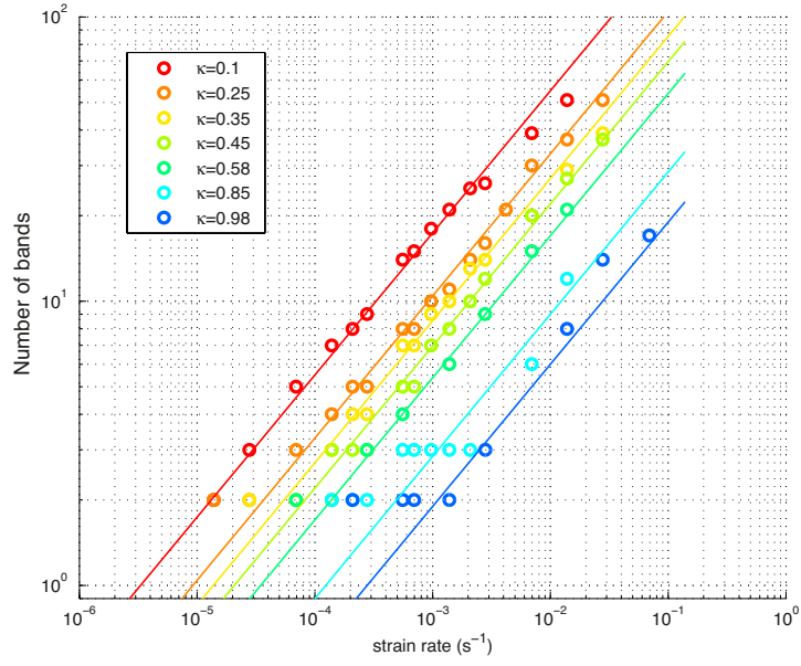
Figure 23: Number of localised band ( N ) vs. strain rate ( \dot{\delta}/L_0 ) in a log-log grid for various nucleation conditions ( \kappa ).
