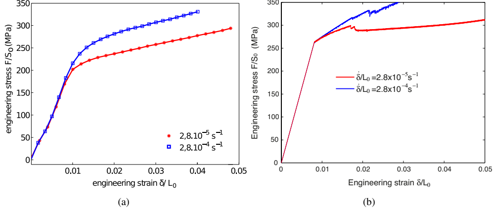
Figure 12: Comparison experiments / modelling: a/b- tensile curves at \dot{\delta}/L_0 = 2.8 \times 10^{-5}; 2.8 \times 10^{-4} \text{ s}^{-1} .
