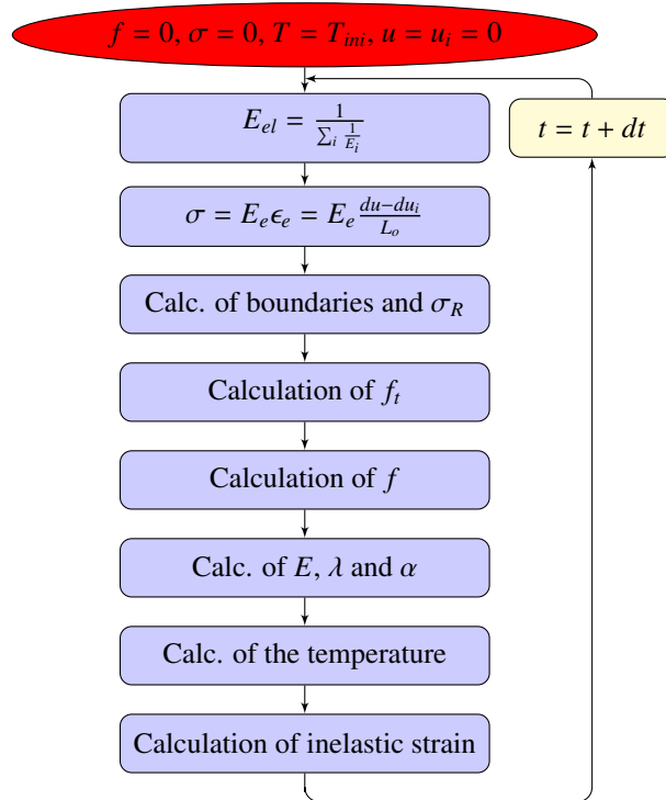
Figure 8: Numerical algorithm for the resolution of the equations associated to the model.
