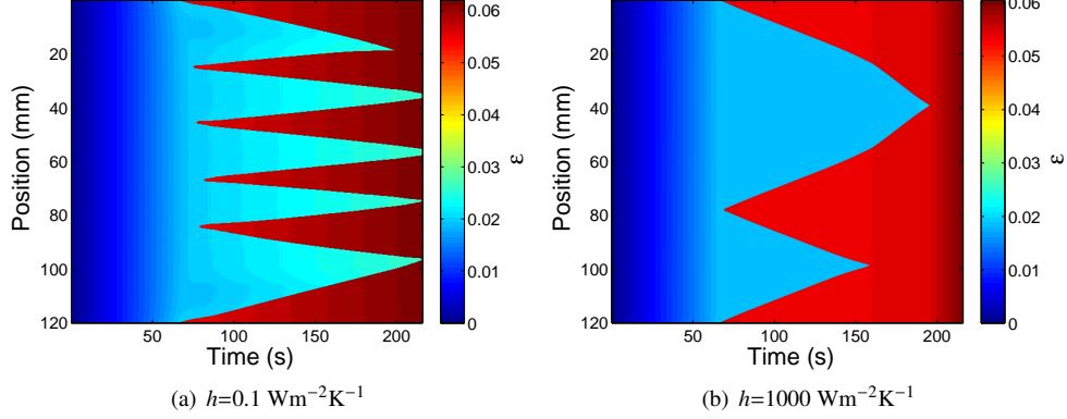
Figure 19: Spatiotemporal evolution of the longitudinal strain at \delta/L_0=2.8 \times 10^{-4} \text{ s}^{-1} : a- low convection coefficient; b- high convection coefficient.
