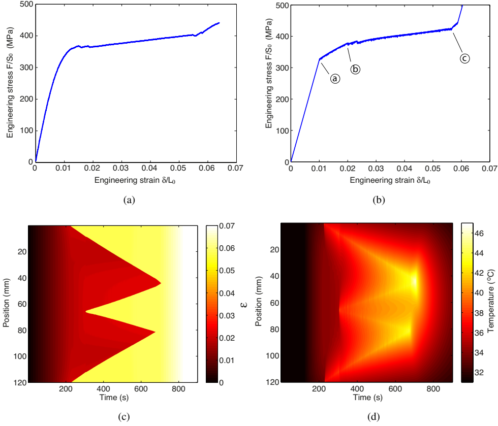
Figure 10: Comparison experiments / modelling: a/b- tensile curves at \dot{\delta}/L_0 = 8.3 \times 10^{-5} \text{ s}^{-1} . c- spatiotemporal map of axial deformation. d- spatiotemporal map of temperature. Dimensions are given in mm.
