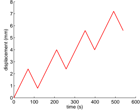
Figure 31: Incremental loading at a constant absolute strain rate \dot{\delta}/L_0 = 4.2 \times 10^{-4} \text{ s}^{-1}
