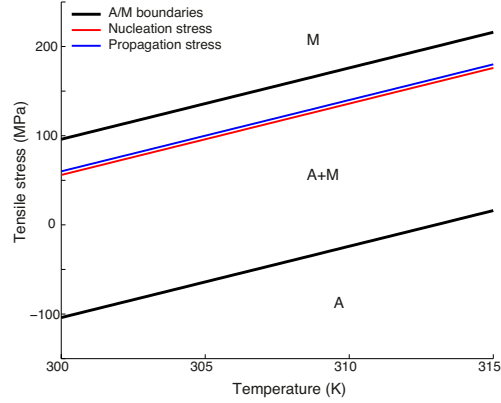
Figure 25: Homogeneous and localisation boundaries for the reverse transformation: from M to A phases.
