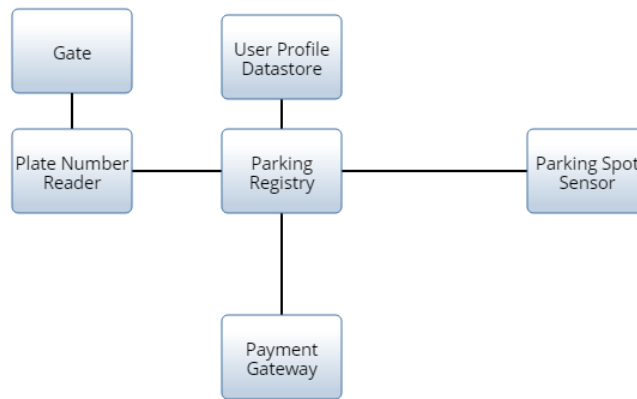
Fig. 6: Assets
