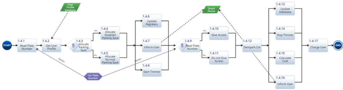
Fig. 5: Functions
