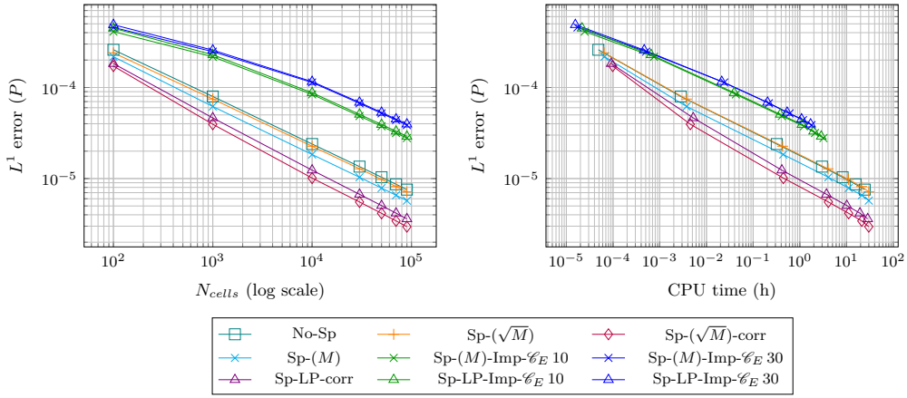
Figure 5: Convergence curve (left), Efficiency curve (right) for the pressure variable p : M = 1.26 \times 10^{-2}
