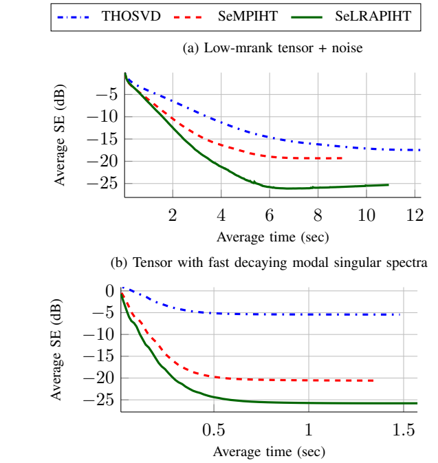
Fig. 1. Performance of IHT algorithms in the completion of a 20 \times 20 \times 20 \times 20 tensor, with target mrank \mathbf{r} = (8, 8, 8, 8) and 5% sampled entries.
