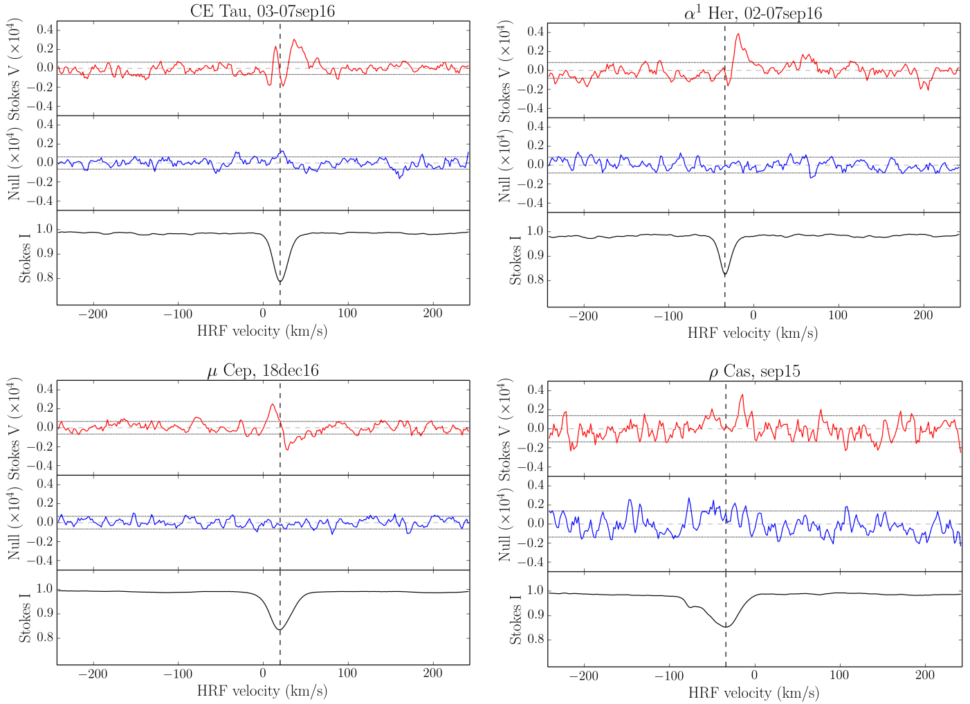
Fig. 1. Highest S/N LSD profiles. For each panel, top plot : Stokes V in red; middle plot : null diagnosis in blue; and bottom plot : Stokes I in black. The dotted horizontal lines represent the \pm 1\sigma level and the dashed horizontal lines the 0 position. The vertical line marks the radial velocity of the star in the heliocentric rest frame. The profile of \mu Cep is free from linear polarisation to circular polarisation cross-talk (see Sects. 3.3 and 3.4.2)
