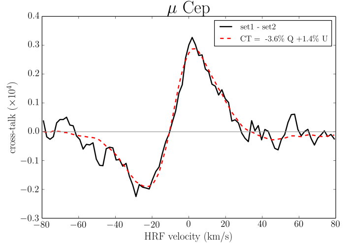
Fig. 4. Least-squares fitting of V_{\text{cross-talk}} on the half-difference between set 1 and set 2 (see Sect. 3.4.2). The black solid line represents the Stokes V resulting from the half-difference and the dashed red line represents the least-squares fit of the cross-talk function. The horizontal line represents 0 level.
