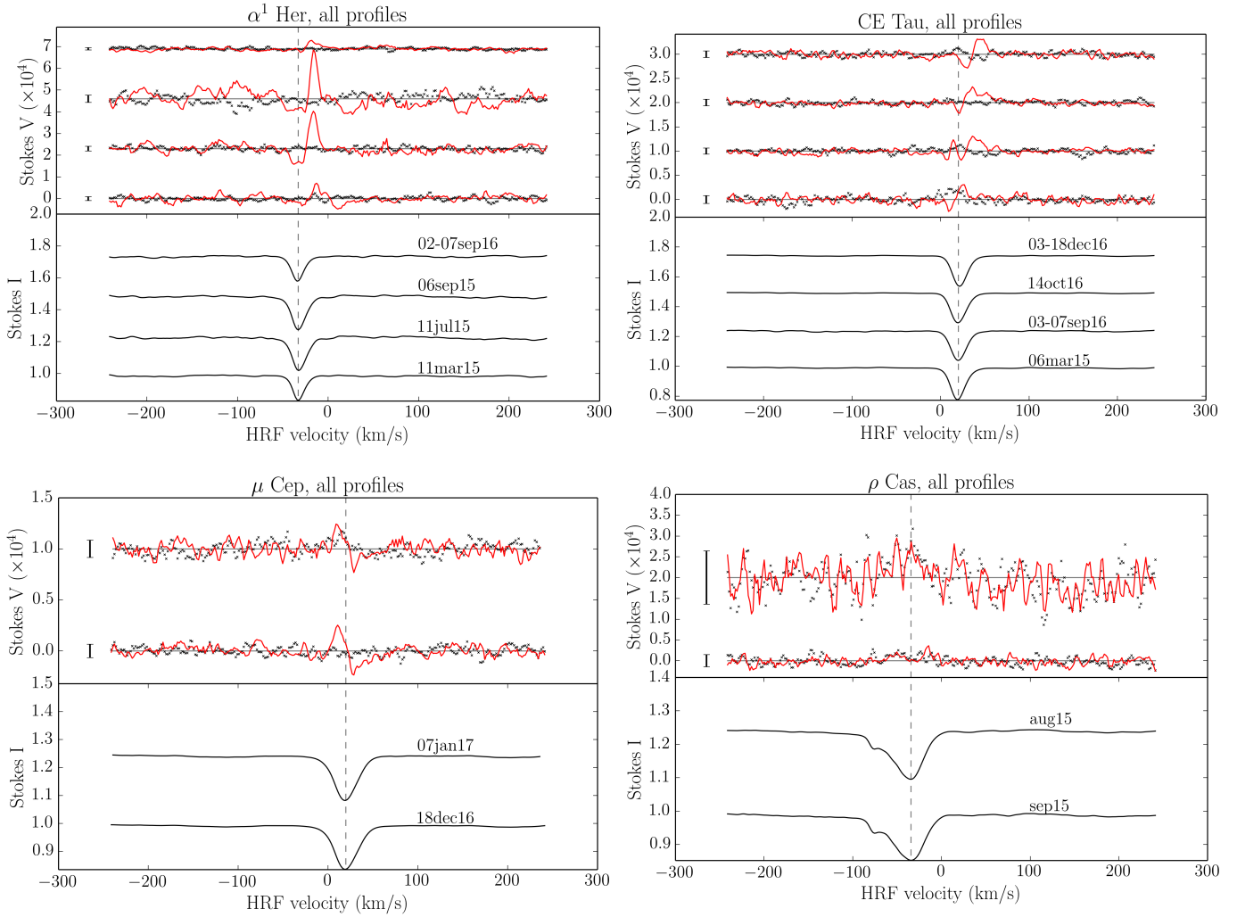
Fig. 5. Variation of the LSD profiles of \alpha^1 Her, \mu Cep, \rho Cas and CE Tau. For each observation point of Table 2, except for \mu Cep, contiguous observations were averaged. For each star, the top panels represent all Stokes V profiles. The bottom panels represent the Stokes I profiles. For each panel the dashed vertical lines mark the mean velocity of the star in the heliocentric rest frame, the horizontal solid lines the position of 0 and the black vertical segments the mean 1\sigma level. The null diagnosis is shown in each panel as black crosses.
