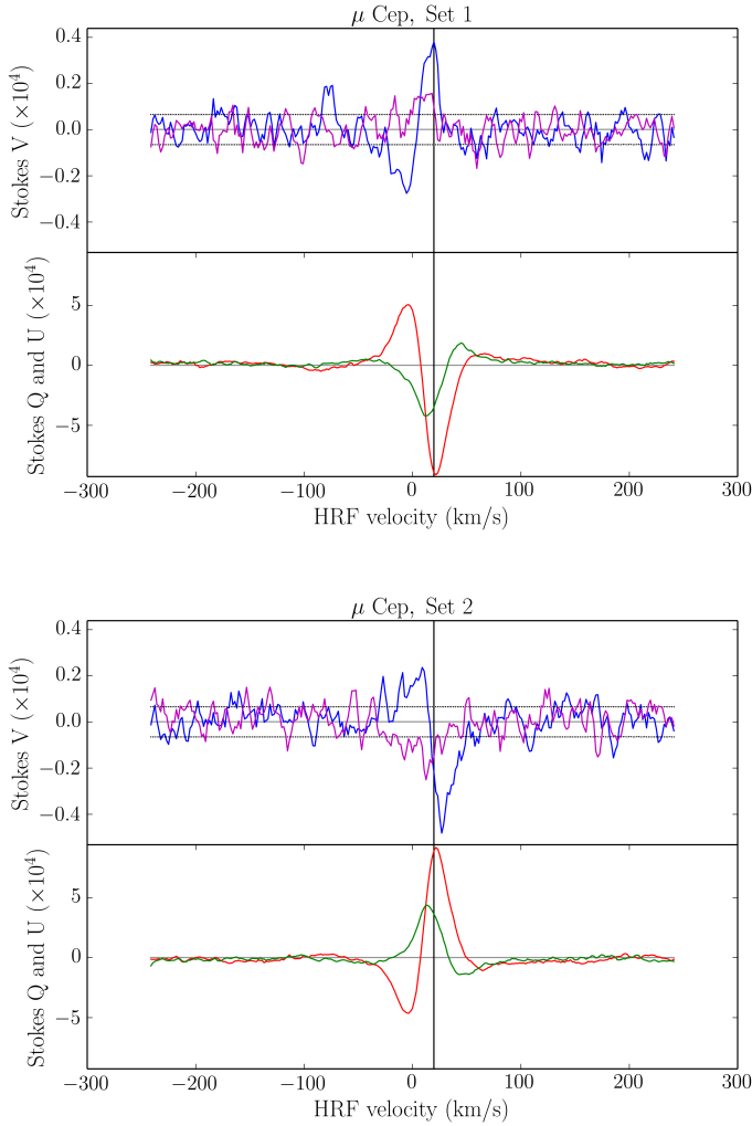
Fig. 2. Mean Stokes V profiles (blue), null diagnosis (purple), Stokes Q (red) and Stokes U (green) profiles for the two sets described in Sect. 3.4.2. Upper panel shows set 1 and lower panel show set 2. The horizontal dotted lines represent the 1\sigma level, the horizontal solid line the 0 level and the vertical line indicates the velocity of the star in the heliocentric rest frame.
