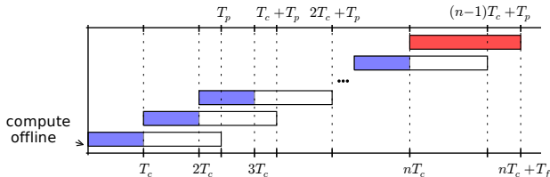
Fig. 1: Receding horizon scheme with termination plan. T_f is both prediction horizon and implementation timeslot for the termination plan in red.
