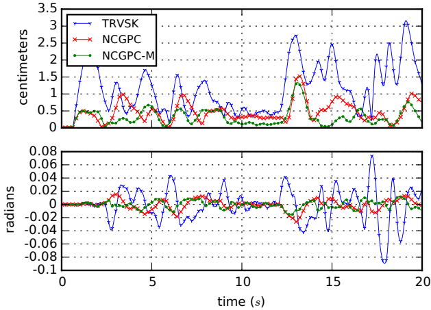
Fig. 6: Errors in position and orientation for the first 20 seconds of the simulation shown in Fig. 5.
