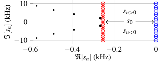
FIG. 4. (Color online) First poles (s_n)_n of \hat{h}_4 , given by (94), for three models. (●): fractional (101). (⊙): EHR (102). (⊕): inviscid, i.e. (102) with a_0 = 0 . Marker area is proportional to residue magnitude |r_n| (95).
