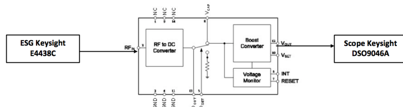
Figure 1 – Measurement platform
