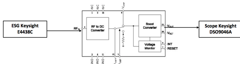
Figure 1 – Measurement platform
