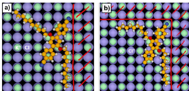
Figure 6. (a) Optimized adsorption geometry for a single CDB molecule at a step edge on the KCl (001) surface. The CN anchoring group simultaneously interacts with two surface cations, while the hydrocarbon chain adsorbs along the step edge itself. (b) The optimized adsorption geometry for a single CDB molecule at a kink feature on the KCl (001) surface. The CN anchoring group simultaneously interacts with three surface cations, while the two hydrocarbon chains lie along the step edges. These interactions contribute to greatly increase the adsorption energy of the molecule.
