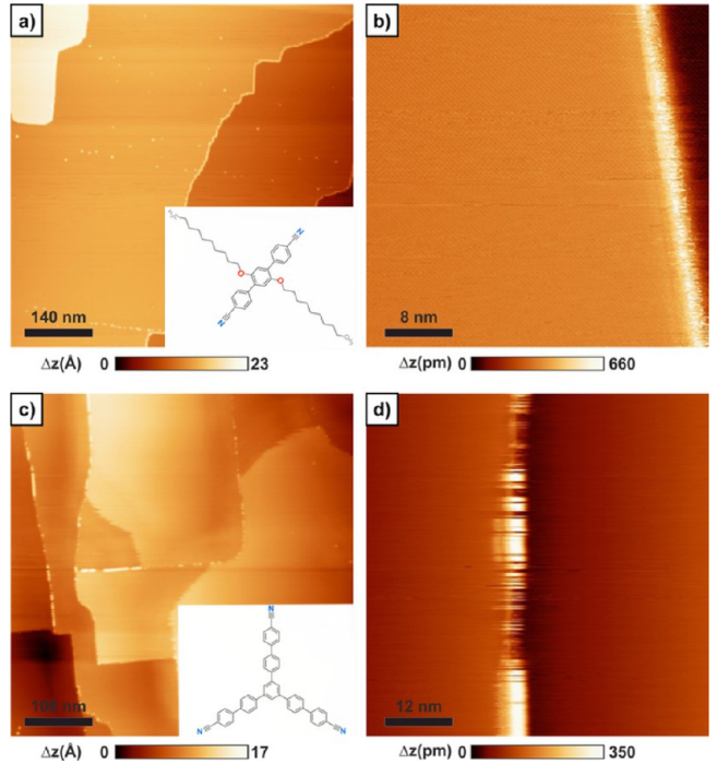
Figure 1. (a) Topography image where 0.05 monolayers (ML) of CDB molecules was deposited onto KCl (001). In the upper left corner there is a terrace, which is completely covered by CDB molecules, and all step edges are fully decorated. (b) A topography image of 0.05 ML of CDB molecules deposited onto KCl (001) showing a decorated step edge. (c) A topography image of TCB molecules deposited onto KCl (001), which shows mostly undecorated step edges and fuzzy stripes. These reproducible fuzzy stripes represent areas where molecules diffuse along crystallographically oriented steps. (d) A representative zoomed-in image over a fuzzy step edge area. A few of the bright objects are stably imaged; however, larger fuzzy stripes can be observed over several scans.
