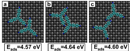
Figure 9. Three stable dimer configurations as observed in MD simulations. Energy minimization calculations were performed to find the energetically lowest geometries. The adsorption energy of a single TCB molecule in the respective configuration is given below each image.
