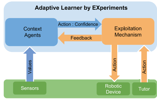
Fig. 1. ALEX architecture.
