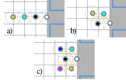
Figure 7: a) Too narrow passage for a biconnectivity. This will be referred to as Tunnel shape a. b) 2-row staggered biconnected formation. (Tunnel shape b.) c) Biconnected formation for larger passages. (Tunnel shape c.).
