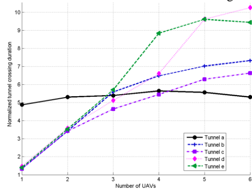
Figure 14: Tunnel crossing duration for each simulated configuration, normalized by the duration of tunnel crossing by a single UAV by the shortest path at maximum speed.
