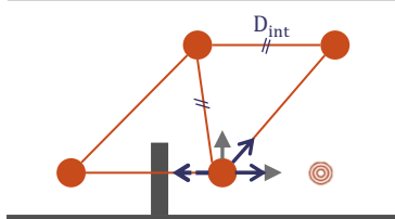
Figure 8: Case when an attractive force is not taken into account (dotted open arrow). The forces are plotted for the UAV of interest.
