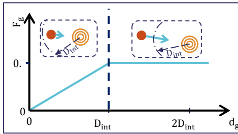
Figure 3: Graphical representation of the attractive force to a goal. The UAV target is represented by nested circles. Note: This notation will be used all along this paper.
