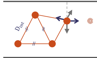
Figure 5: Scheme of the repulsive and attractive forces applied to a UAV in a swarm, in a narrow passage.
