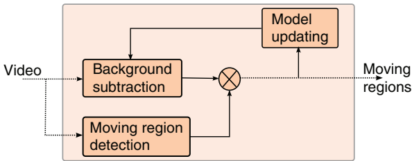
Fig. 3 Synopsis of the motion detection module.
