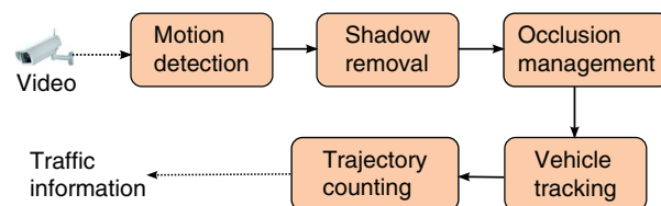
Fig. 2 Synopsis of the proposed system for vehicle counting.
