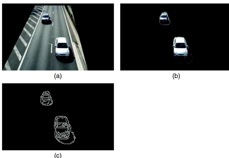
Fig. 7 Foreground edges: (a) observed scene, (b) moving region detection result, and (c) detected edges.
