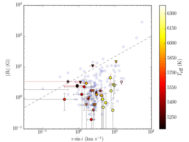
Figure 4. Plot of the maximum measured |B_{\ell}| versus v \sin i for the planet-hosting stars (symbols are as in Fig. 1). Stars located above the dashed line have significantly higher |B_{\ell}| than others with similar v \sin i , as per Marsden et al. (2014, section 6.3.3). The complete BCool sample is shown as blue circles.
