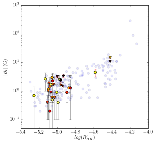
Figure 6. Plot of maximum measured |B_\ell| versus \log(R'_{HK}) (Table 8) for the planet-hosting stars. Symbols are as in Fig. 1. The complete BCoolest sample is shown as blue circles.
