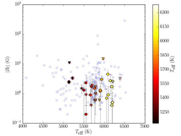
Figure 3. Plot of the maximum measured |B_{\ell}| versus T_{\text{eff}} for the planet-hosting stars (symbols are as in Fig. 1). The complete BCool sample is shown as blue circles.
