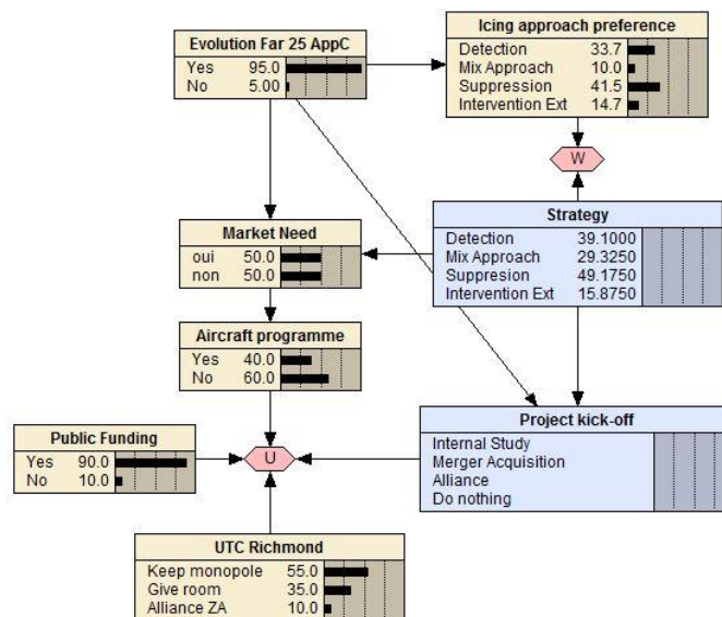
Fig.4 - Influence diagram - Phase 1 decision situation
