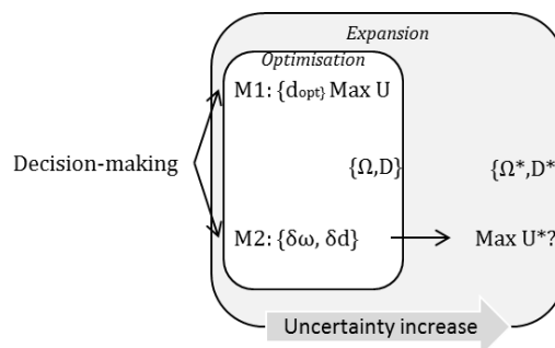
Fig. 2 - Optimisation vs. Expansion
