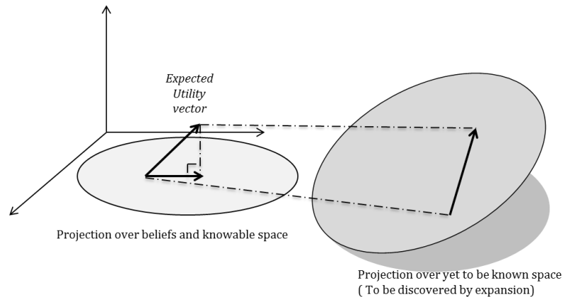
Fig.3 - Projection vs. Expansion
