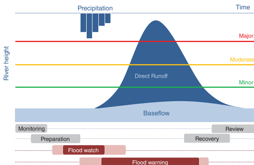
FIGURE 2 | The stages of a flood event. Heavy precipitation (top) precedes the rise of the river level (middle). The level may exceed various flood impact thresholds (e.g., minor flooding is the inundation of low-lying farm lands whereas major flooding may affect buildings and other structures). Various products and modes of operation (bottom) are discussed in the text.
