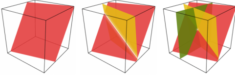
Fig. 8: Secret sharing through hyperplan intersection
