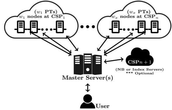
Fig. 15: SSSS-based framework [67, 66, 100, 65]
