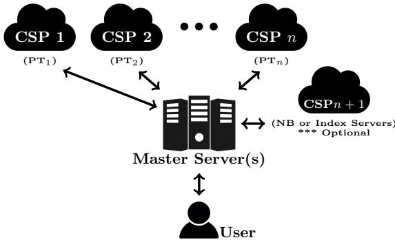
Fig. 14: Architecture from [6,5,32,63]
