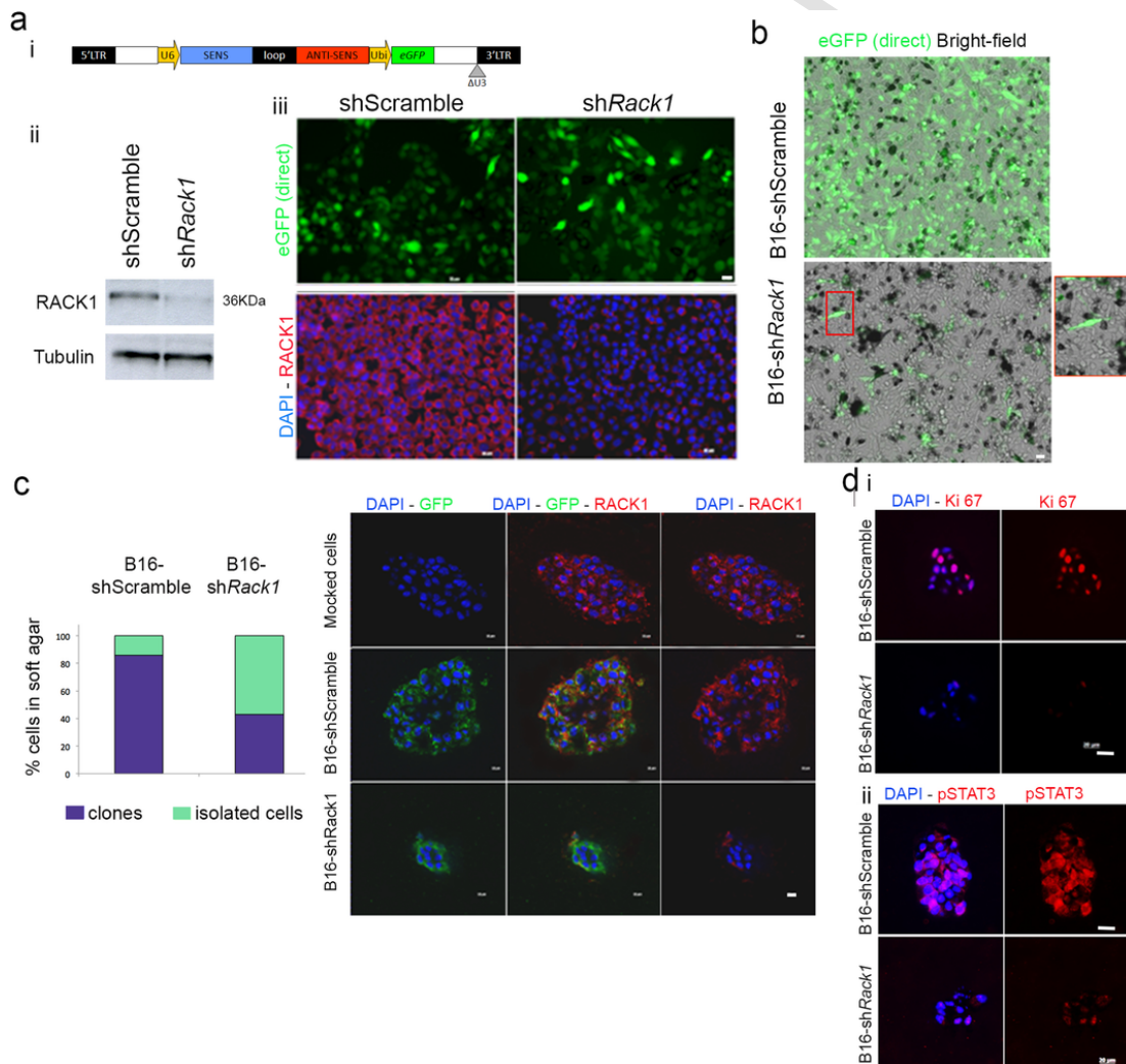
Fig. 1. RACK1 knock-down reduced B16 melanoma cells invasiveness and led to cell differentiation. a: i) Lentiviral vector backbone for shRNA expression with GFP control of transduction; ii) Western-blot analysis for RACK1 and Tubulin in shRack1 and shScramble B16 cells 3 days post-transduction (3dpt); iii) Fluorescent microscopy analysis of direct GFP signal (green) and immunolabeling for RACK1 (red) on 3 day-transduced cells. b: Aspect of shRack1 and shScramble -treated B16 cultures 14 days after transduction. Note the differentiation and loss of GFP + cells in shRack1 -treated B16 cells. c: Soft agar assay of shRack1 and shScramble -treated B16 cells 3dpt, i) Proportions of clones (purple) and isolated cells that did not proliferate (green); ii) Immunolabeling for GFP (green) and RACK1 (red) in B16 clones mock-treated or treated with shRack1 or shScramble ; d: Immunolabeling for i) the proliferation marker Ki67 (red) or ii) pSTAT3 (red) on soft agar clones. Nuclear counterstaining with DAPI (blue). Bars: 20 \mu m. (For interpretation of the references to colour in this figure legend, the reader is referred to the web version of this article.)
