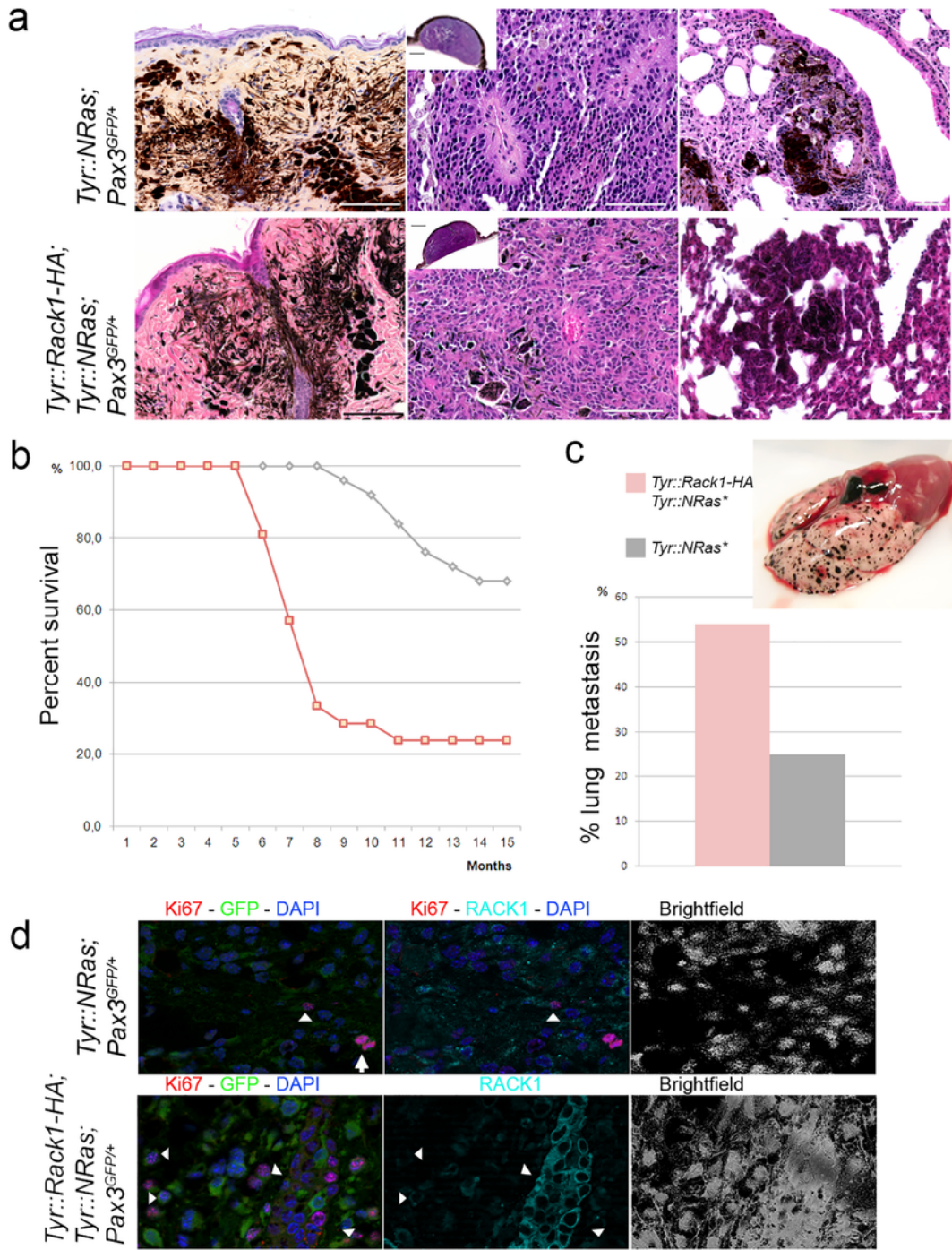
Fig. 4. Targeted RACK1 overexpression reduces latency and increases incidence of melanoma development in Tyr::NRas* mice. a , Histological features (haematoxylin-eosin-saffron staining) of melanocytic nevi, primary cutaneous melanoma and lung metastases in Tyr::NRas* ; Cdkn2a +/- ; Pax3 GFP/+ mice and Tyr::Rack1-HA ; Tyr::NRas* ; Cdkn2a +/- ; Pax3 GFP/+ mice. Note that lesions are histologically indistinguishable among groups. b , Survival (Kaplan-Meier plot) for Tyr::Rack1-HA ; Tyr::NRas* ; Pax3 GFP/+ mice (n = 22, pink curve) compared to Tyr::NRas* ; Pax3 GFP/+ control mice (n = 25, grey curve). Mice from the three transgenic lines were pooled in the Kaplan-Meier graph. c , Percentages of lung metastases in Tyr::Rack1-HA ; Tyr::NRas* ; Pax3 GFP/+ mice (pink bar) compared to control Tyr::NRas* ; Pax3 GFP/+ (grey bar). Gross feature of a Tyr::Rack1-HA ; Tyr::NRas* ; Pax3 GFP/+ lung with multiple melanoma metastases. d , ApoTome microscopy analysis of double labeling for Ki67 (red), GFP (green) and RACK1 (cyan) in control Tyr::NRas* ; Pax3 GFP/+ mice and in Tyr::Rack1-HA ; Tyr::NRas* ; Pax3 GFP/+ mice. Nuclear counterstaining in blue. Bars: 10 \mu m. Arrowheads point to Ki67 + , GFP + , RACK1 + melanocytic cells. Arrow points to a mitosis, RACK1 - . In the lower row, intense RACK1 + cells are keratinocytes. (For interpretation of the references to colour in this figure legend, the reader is referred to the web version of this article.)
