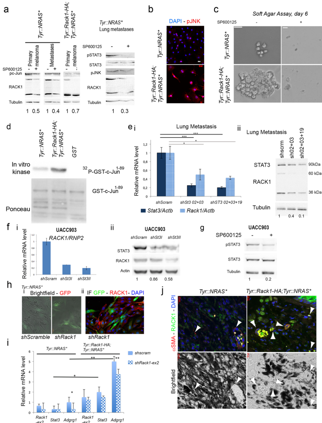
Fig. 6. RACK1 regulation and angiogenesis in melanoma. a , Western blot analysis of pc-Jun and RACK1 after SP600125 inhibition of JNK on protein lysates from primary melanoma and metastases from Tyr::NRAS* ; Pax3 GFP/+ mice and primary melanoma cells in Tyr::Rack1-HA ; Tyr::NRAS* ; Pax3 GFP/+ . SP600125 20 \mu M reduced RACK1 levels after 48 h treatment. pc-Jun reduction is shown. Western blot analysis of RACK1, pSTAT3, STAT3 and pJNK, in Tyr::NRAS* ; Pax3 GFP/+ melanoma lung metastatic cells after treatment with 20 \mu M SP600125 for 48 h and quantification. b , pJNK immunoreactivity on cells from primary melanomas of Tyr::Rack1-HA ; Tyr::NRAS* ; Pax3 GFP/+ mice compared to the ones from Tyr::NRAS* ; Pax3 GFP/+ mice. Bars: 10 \mu m. Note a higher pJNK signal on Rack1 overexpressing cells. c , Soft agar assay over 6 days with melanoma cells overexpressing Rack1-HA and controls without or with SP600125 (20 \mu M). Rack1-HA cells started forming clones earlier, and SP600125 prevented it. Bars: 10 \mu m. d , In vitro JNK kinase assay. Cell lysates from Tyr::NRAS* ; Pax3 GFP/+ and Tyr::Rack1-HA ; Tyr::NRAS* ; Pax3 GFP/+ melanomas and Tyr::NRAS* ; Pax3 GFP/+ melanocytes were subjected to immunoprecipitation using JNK antibody followed by kinase assay using GST-c-Jun 1-89 as substrate. e , i , Quantitative RT-PCR for Stat3 (dark blue bars) and Rack1 (hatched light bars) mRNAs on lung melanoma metastasis cells after treatment with lentiviral vectors coding for shStat3 (02, 03, 19) or control. Results shown are Stat3 or Rack1 expression normalized to Actb from triplicates. * P < 0.05 , *** P < 0.001 . ii , Western-blot for RACK1, STAT3 and Tubulin after Stat3 knock-down on mouse melanoma cells. f , i , Quantitative RT-PCR for RACK1 mRNA on human UACC903 melanoma cells after treatment with lentiviral vectors expressing shSTAT3 or shScramble . RACK1 levels are normalized to RNP2 . e , ii , Western-blot for RACK1, STAT3, and Actin after STAT3 knock-down. g , Western blot analysis for
