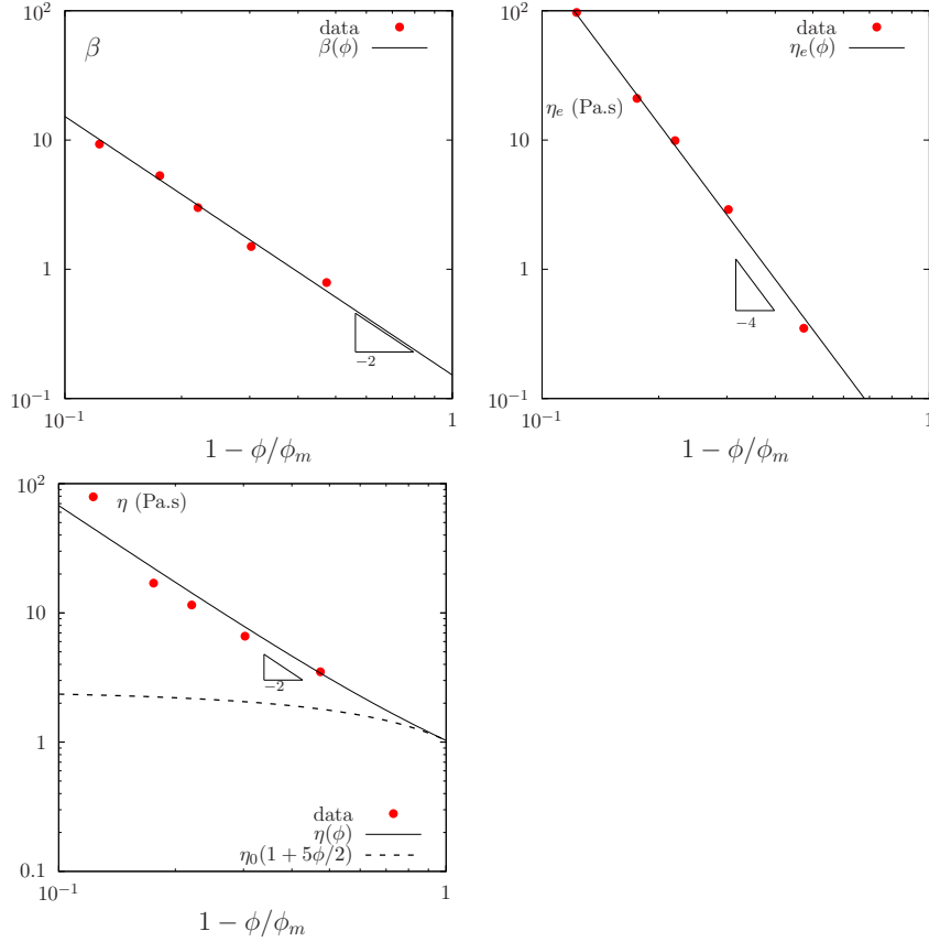
FIG. 11. Evolution with \phi of the model parameters \beta , \eta_e , and \eta , and best fits provided by expressions (16a)-(16c).
