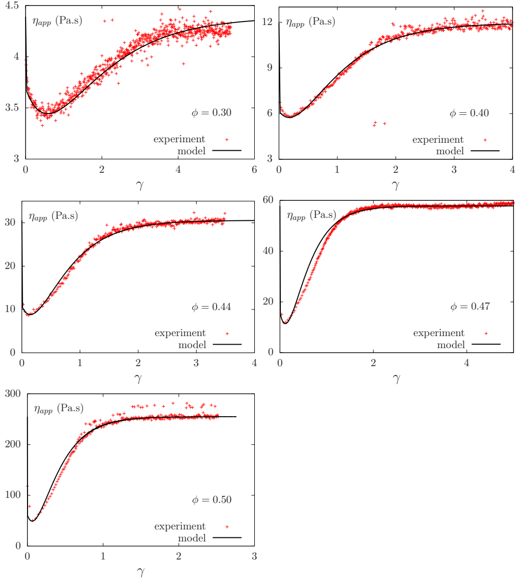
FIG. 10. Shear reversal: apparent viscosity \eta_{app} vs deformation \gamma . Comparison between experimental measurements from Blanc (2011) for a suspension of PMMA particles in a Couette geometry and computations with the present model. For each volume fraction \phi , the three model parameters \beta , \eta_e , and \eta were obtained through a best-fit procedure. Parameter values are indicated in Table II .
