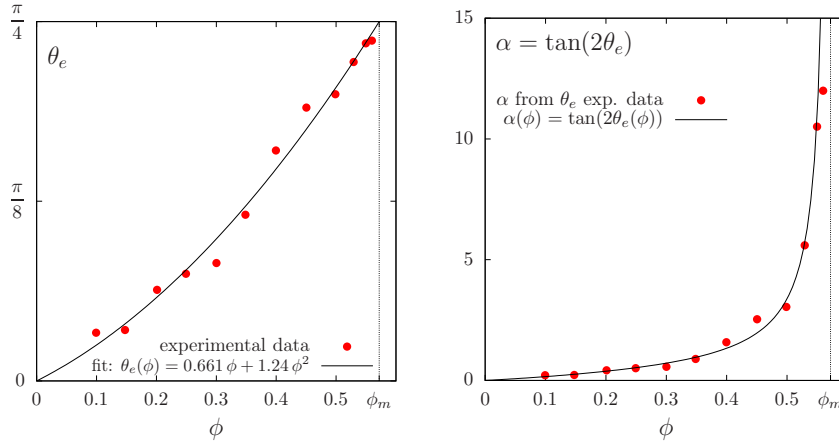
FIG. 2. (left) Depletion angle \theta_e versus volume fraction \phi : experimental data from Blanc (2011), Fig. 5.11, and best fit with the second-order polynomial (10). (right) Dependence upon \phi of model parameter \alpha .
