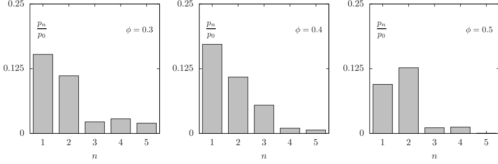
FIG. 5. Five first Fourier coefficients p_k , k \geq 1 of the probability distribution function p(\theta) , from experimental data by Blanc (2011), Fig. 5.10, for \phi = 0.3, 0.4 and 0.5 .
