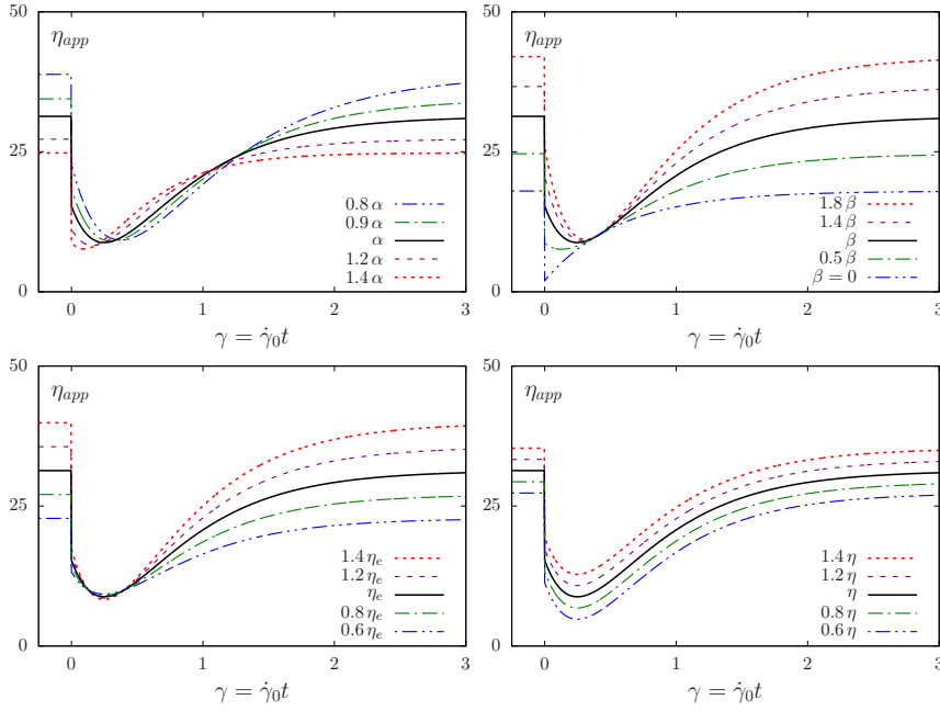
FIG. 9. Apparent viscosity during shear reversal: sensitivity of the response to the model parameters (base value of the parameters: \alpha = \sqrt{3} , \beta = 5 , \eta_e = 10 Pa.s, \eta = 10 Pa.s).
