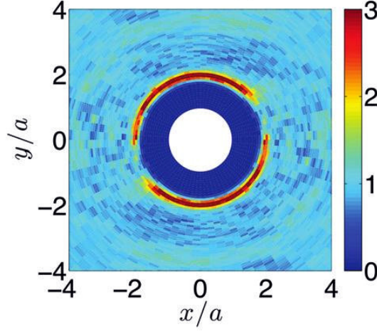
FIG. 3. Pair distribution function g(x, y) : experimental observation by Blanc et al. (2013) for a stationary shear flow with \phi = 0.35 .
