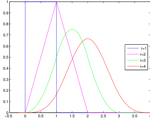
Figure 3: Spline functions \varphi^{(r)}
