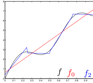
Figure 2: Example of approximation by piecewise linear functions
