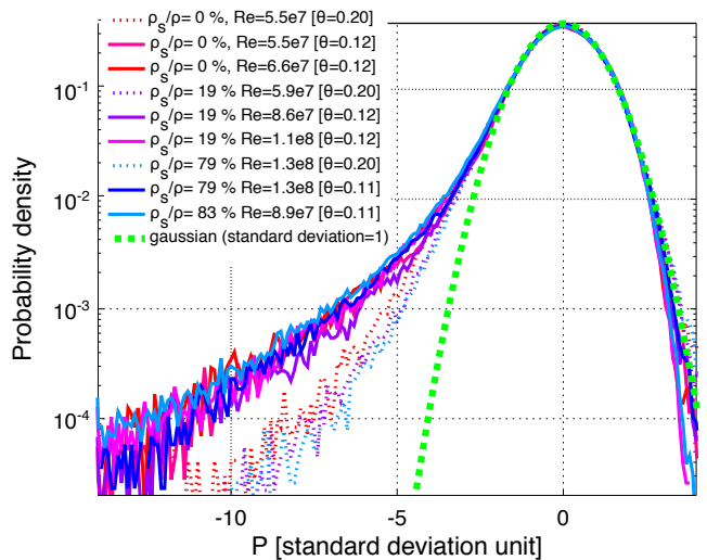
Fig. 3: Probability density function (pdf) of the pressure fluctuations normalized to unity standard deviation.
