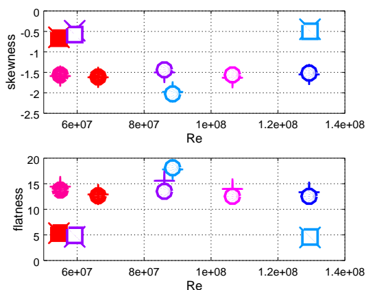
Fig. 4: Upper (lower) plot : skewness (flatness) of pressure fluctuations. The open (full) symbols correspond to measurements in superfluid (in classical liquid helium). The square-shaped (circle-shape) symbols are for a differential rotation parameter of \theta = 0.2 ( \theta = 0.11 - 0.12 ). The crosses and pluses symbols correspond to the probe-bandwidth check with 53Hz low-pass filtering (see text).
