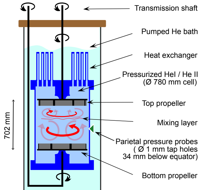
Fig. 1: Schematic of the experiment.
