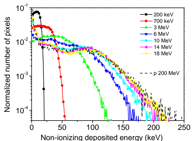
Figure 7: Non-ionizing deposited energy events recorded in an array of pixels, for different energies of incident neutrons.
